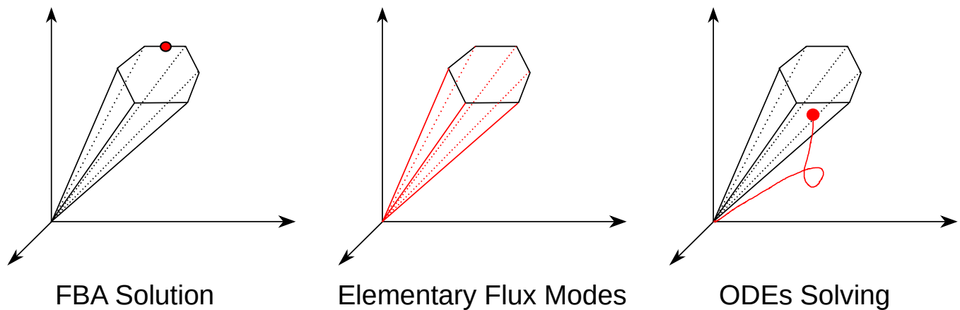
Figure 2.8: Constraint-based modelling in a nutshell: Steady-state modelling: FBA, EFMs vs. Dynamic Modelling
