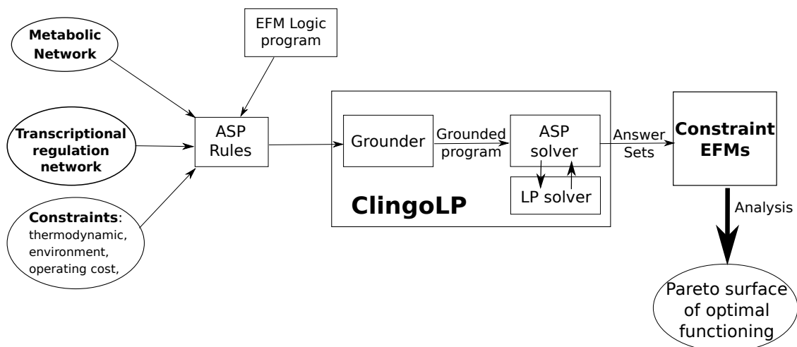
Figure 3.3: Schematic overview of the aspefm workflow for computing EFM under constraints. The ASP rules representing the metabolic model and additional biological constraints are given as input into clingo [LP] along with the logic program for computing EFM. From all of these rules, the grounder of clingo [LP] generates instantiated constraints, which are sent to the ASP/LP solver. The resulting answer sets are EFM consistent with all the constraints. These EFM can be analyzed in post-processing to select the optimal functioning ones.
