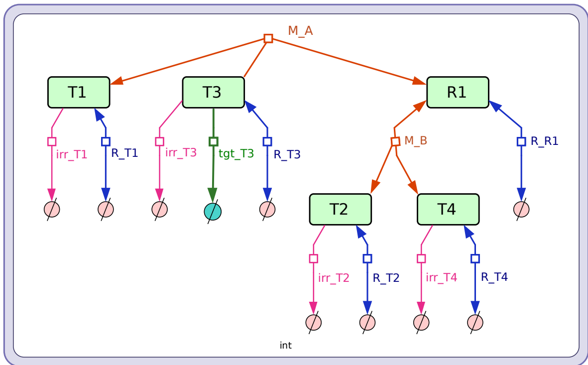
Figure 2.18: MCSs dual network of the toy model, using Ballerstein's formulation
