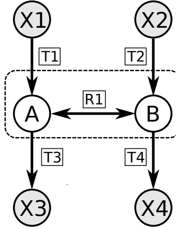
Figure 2.7: Toy model network of 5 reactions
