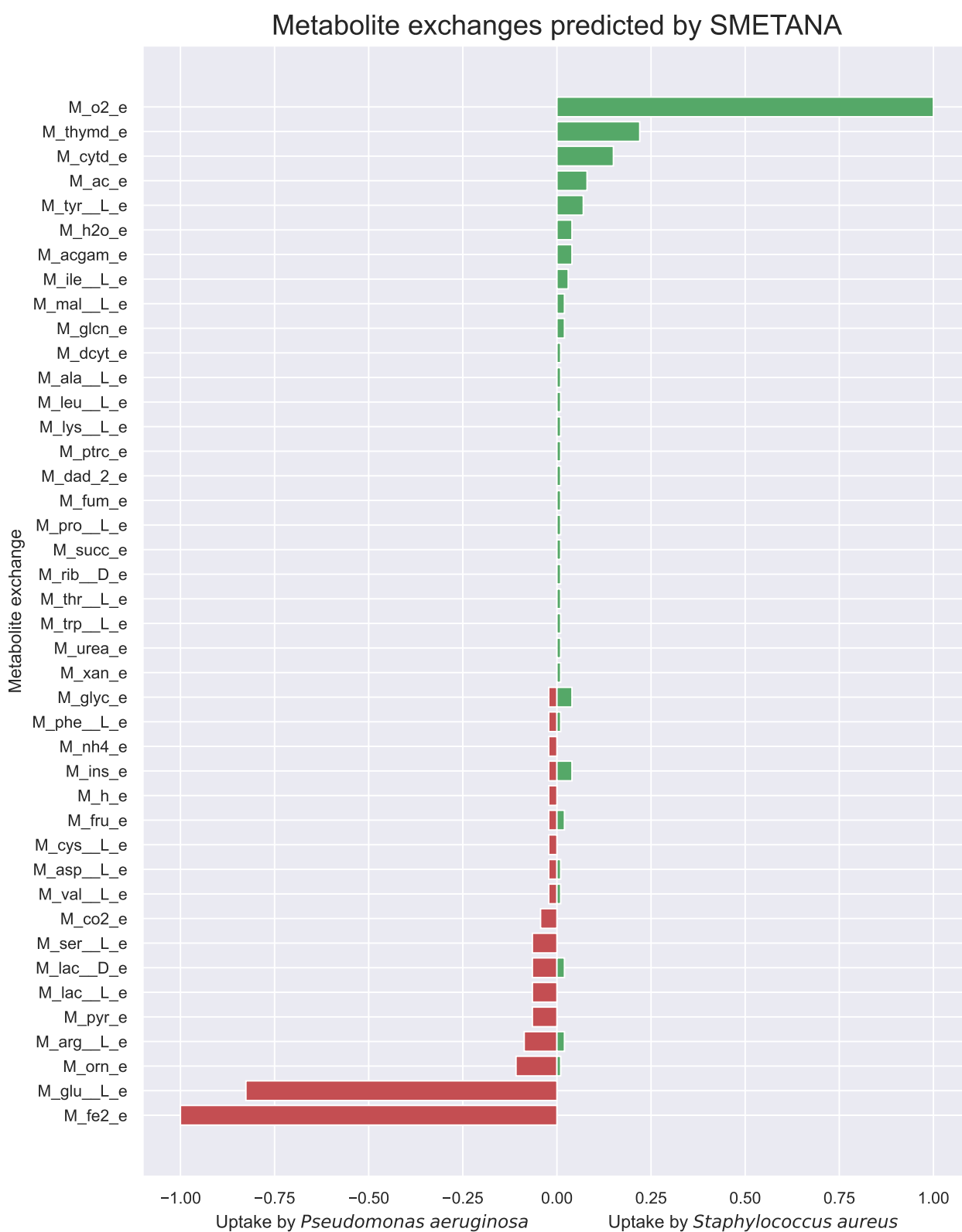
Figure 4.15: Estimated potentials for metabolite exchanges between the two bacteria according to SMETANA. Abscissae are SMETANA scores, multiplied by -1 when S.A. is the donor instead of P.A.
