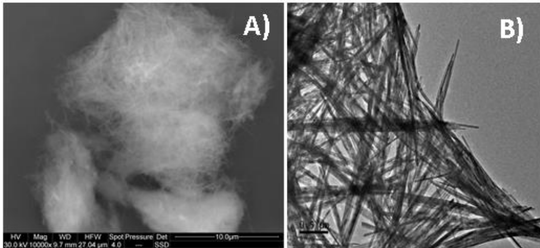
Figure III.7: SEM (A) and TEM (B) images of aggregated xonotlite fibers.
