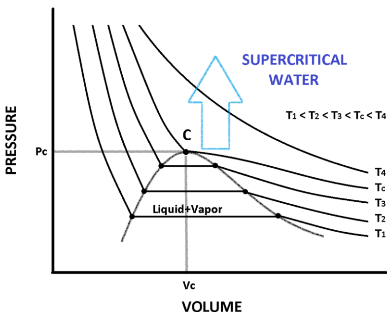
Figure 1.18: Pressure- Volume diagram of water. Note: C points indicates the critical point of water.
