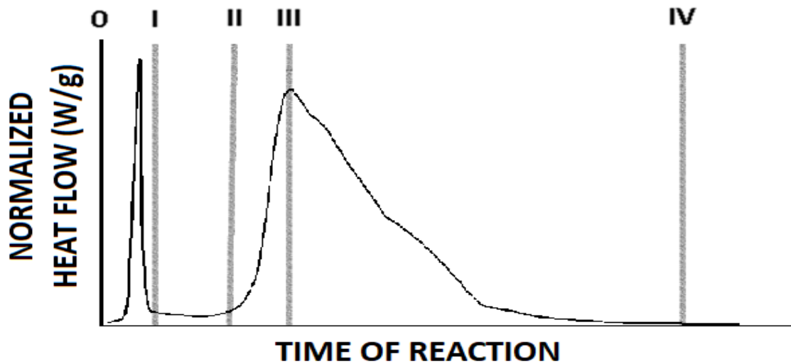
Figure 1.3: Isothermal calorimetry curve with characteristic five steps of cement hydration.
