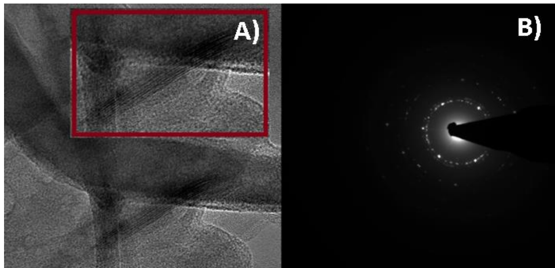
Figure IV.16: High magnification images of tobermorite pristine (A), SAED images of the same sample (B).
