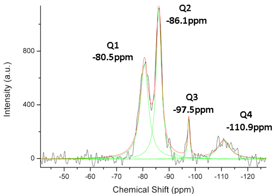
Figure III.28: ^{29}\text{Si} NMR curve of SBS functionalized xonotlite obtained after 4 hours of reaction (xonotlite_SBS 4h). Notes: black curve is the experimental, red curve is the adjusted curve and green curve represents the deconvoluted curves of each signal adjusted to pseudo-Voigt.
