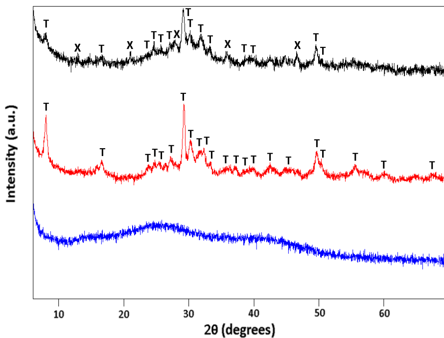
Figure V.11: XRD patterns of pristine tobermorite synthesized at different residence times: 4 seconds (blue curve), 4.3 seconds (red curve) and 6.3 seconds (black curve).
