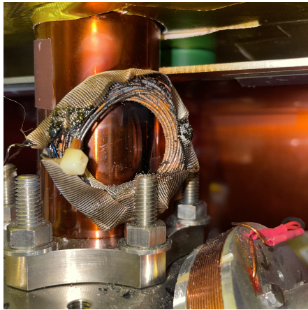
FIGURE III.37: The state of the Stern-Gerlach when the magnetic-shield are opened.
