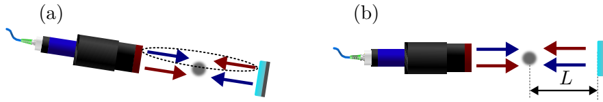
FIGURE V.1: Retro-reflected Raman lasers configuration. (a) Simple diffraction where only one pair (dashed circle) verifies the resonance condition (Doppler effect). (b) Double diffraction configuration where both pairs are resonant.
