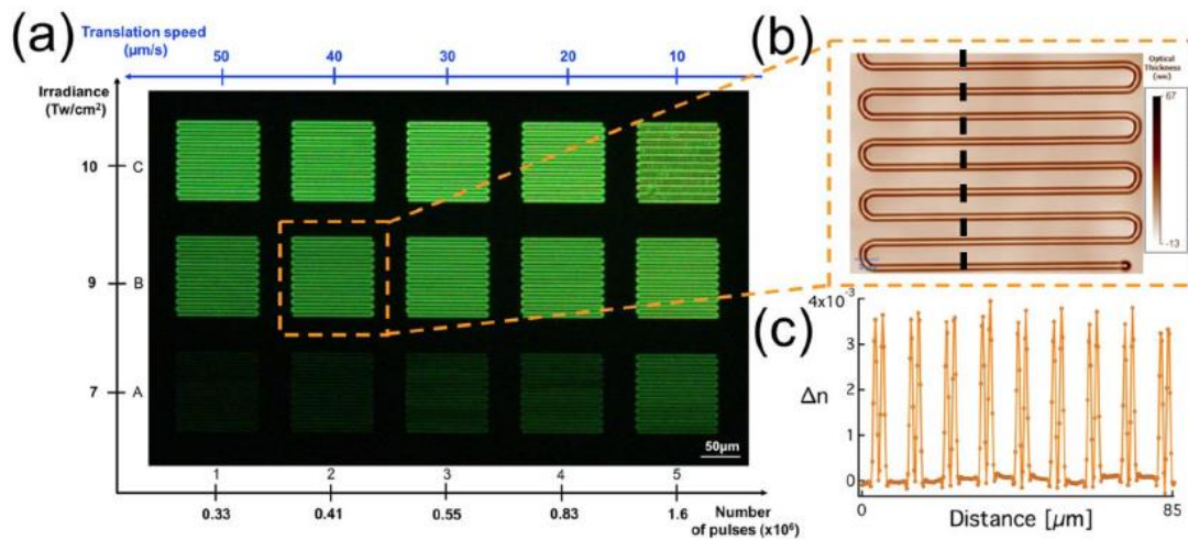
Figure II-12: (a) Fluorescence image ( \lambda_{ex} = 480 \text{ nm} , \lambda_{em} = 550 \text{ nm} ) of the inscribed cartography of the serpentine structures while varying the writing irradiance (along the vertical axis) and the number of pulses (along the horizontal axis) (b) Pop-up of the phase image of one of the structures, acquired through the SID4-Bio device (c) Line profile of positive refractive index change associated with the double-track Type-A structures. Such line profile is extracted from a horizontal cross-section of the structure (dashed black line in (b)). Taken from [156].
