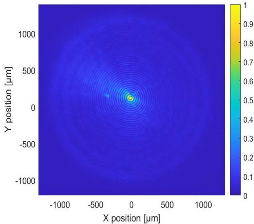
Figure IV-15: Experimental image profile of the intensity cross-section of the Gaussian-Bessel beam close to the \frac{z_{max}}{2} region.
