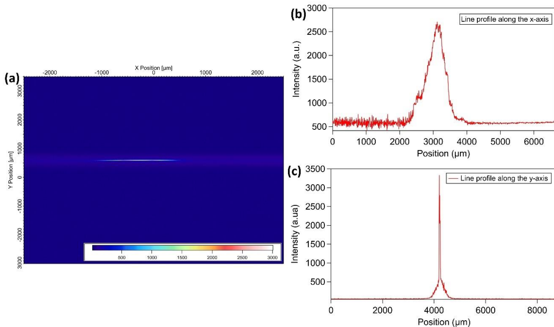
Figure IV-28: (a) Experimental image profile of the produced light-sheet beam. Intensity distribution along the (b) x-axis and (c) y-axis.
