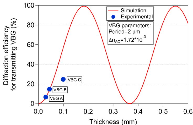
Figure IV-21: Simulated dependence of the diffraction efficiency for transmitting Bragg grating versus VBG's thickness for \lambda=632.8 \text{ nm} , \Delta n_{AC} = 1.72 \times 10^{-3} , \Lambda=2 \mu\text{m} .
