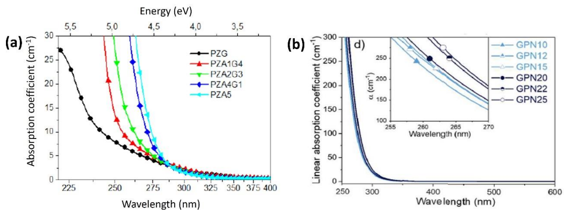
Figure II-3: Absorption spectra in UV-Visible range of (a) zinc-phosphate glasses (PZG) containing and non-containing silver ions (Image from [141]), and of (b) silver-containing sodium-gallium phosphate glasses (GPN) (Image from [13]).
