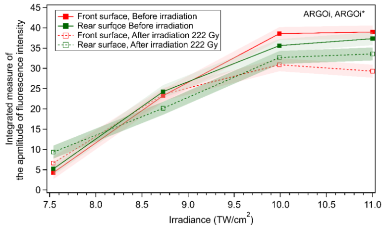
Figure III-30: Integrated measure of the fluorescence amplitude for the different laser irradiances before and after the 222 Gy dose for the two planes in ARGOi and ARGOi* glass sample, under 365 nm excitation.
