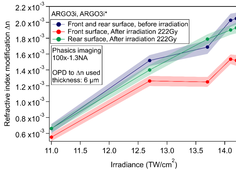
Figure III-34: The refractive index modification \Delta n as a function of laser irradiance before/after 222 Gy-dose for the two planes in ARGO3i, ARGO3i* glass samples.
