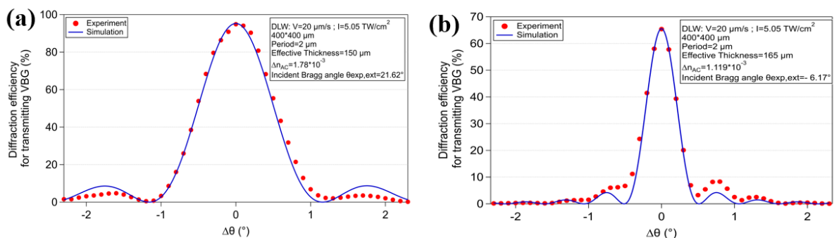
Figure IV-23: Experimental and simulated dependence of the diffraction efficiency from the Bragg angle of the transmitting Bragg grating for \lambda=632.8 \text{ nm} . (a) Incident Bragg angle at 21.62^\circ (first order), (b) incident Bragg angle at -6.17^\circ (second order).
