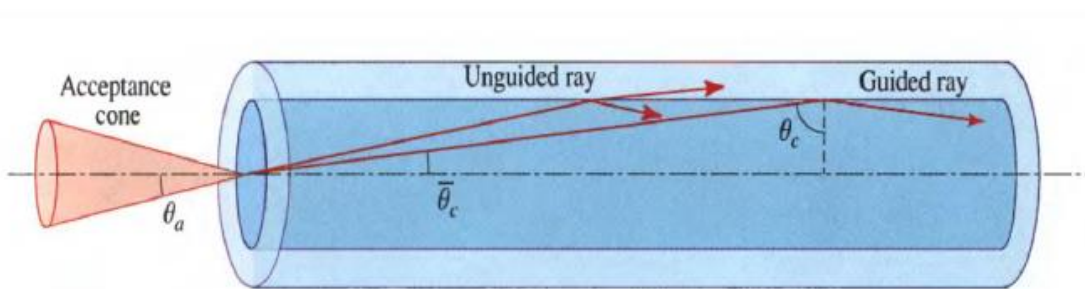
Figure A-2: Schematic representation of an optical fiber with rays within the acceptance cone (defining by the NA) being guided within the fiber by total internal reflection. Taken from [332].
