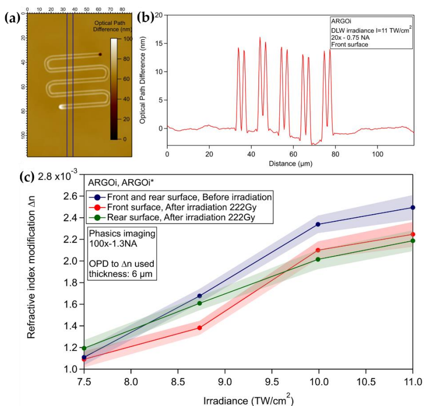
Figure III-28: (a) Phase image under white light illumination of the laser inscribed structure ( 11 \text{ TW}/\text{cm}^2 ) before irradiation. (b) Optical path difference determined from the phase image. (c) Refractive index modification \Delta n as a function of laser irradiance before/after 222 Gy-dose for the two planes in ARGOi, ARGOi* glass sample.
