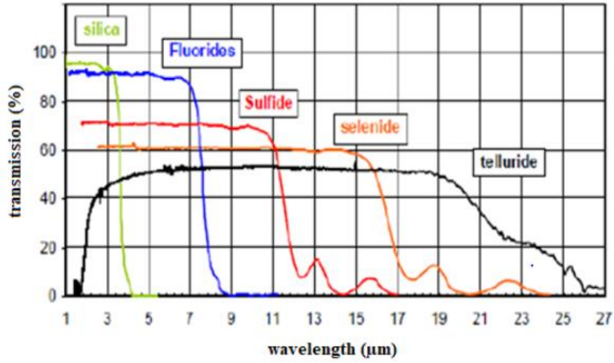
Figure I-5: Absorption spectrum of silica, fluoride and chalcogenide glasses. Taken from [17].
