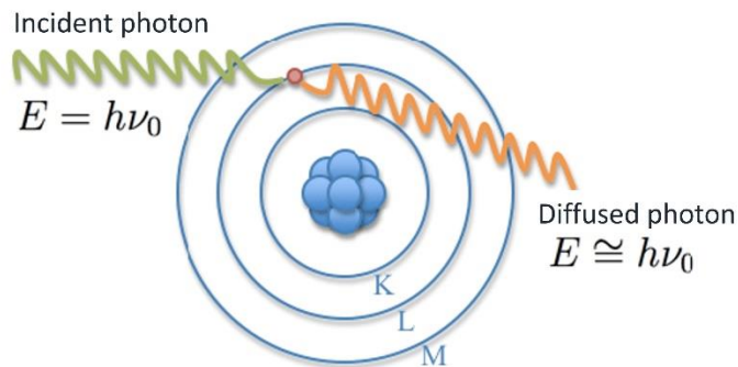
Figure III-7: Representative scheme of Rayleigh diffusion. Taken from [180].
