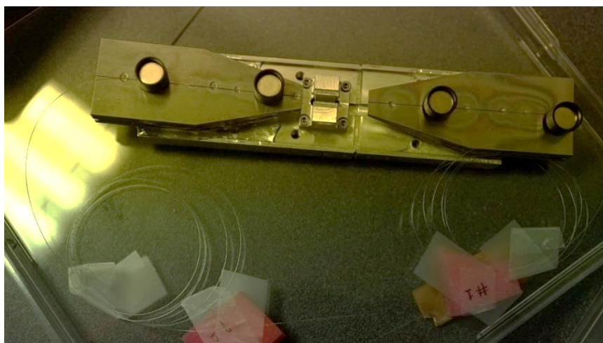
Figure III-46: The ultimate result of the manufactured device for the 5-pass waveguide after connectorization with radiation hardened fibers for the perspective of in-situ radiophotoluminescence and radiation-induced attenuation.
