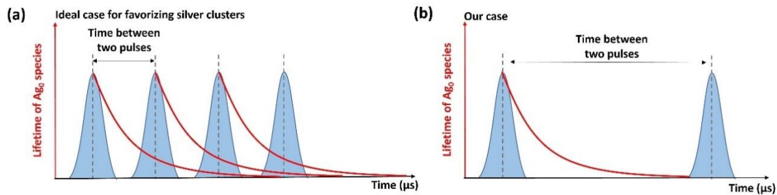
Figure IV-33: Diagram illustrating the decay in the lifetime of Ag^0 species versus the time interval between pulses: (a) an ideal case that promotes the formation of silver clusters, (b) the case observed in our experiment.
