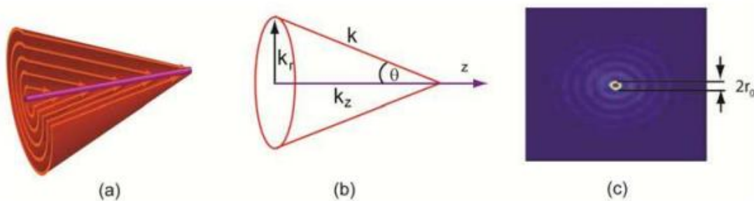
Figure I-14: Schematic representation showing Gaussian-Bessel beam characteristics. (a) The conical flow of energy inwards towards the central lobe of the beam. (b) Demonstration of the relationship between the wave vectors that form a non-diffracting Bessel beam. (c) The
