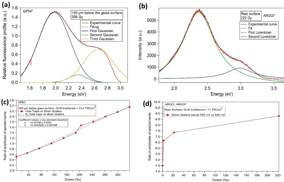
Figure III-39: (a) Fit of the RPL spectra of the GPNi* glass for the laser inscribed structure at 150 μm below the glass surface at 356 Gy X-ray dose. (b) Fit of the RPL spectra of the ARGOi* glass for the highest DLW irradiance structure of the rear surface at 222 Gy X-ray dose. (c) Dose-dependent evolution of the amplitude ratios of extracted spectral bands of the hole trap center Ag^{2+} at 620 nm over the silver clusters Ag_m^{x+} band at 460 nm for the GPNi* glass sample for DLW irradiance of 13.4 TW/cm 2 at 160 μm below the glass surface. (d) Case of the ARGOi and ARGOi* glass sample for DLW irradiance of 11 TW/cm 2 at 550 μm below the glass surface (rear surface) for ratio of the two silver cluster bands (namely, the 525 nm band over the 420 nm band).
