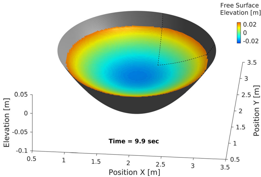
Fig. 9 Free surface elevation of oscillation in parabolic basin with grid nesting after 4.5 cycles (9.9s). The refined Child grid is denoted by the dashed line and shows a more detailed run-up limit than the coarse Parent grid
