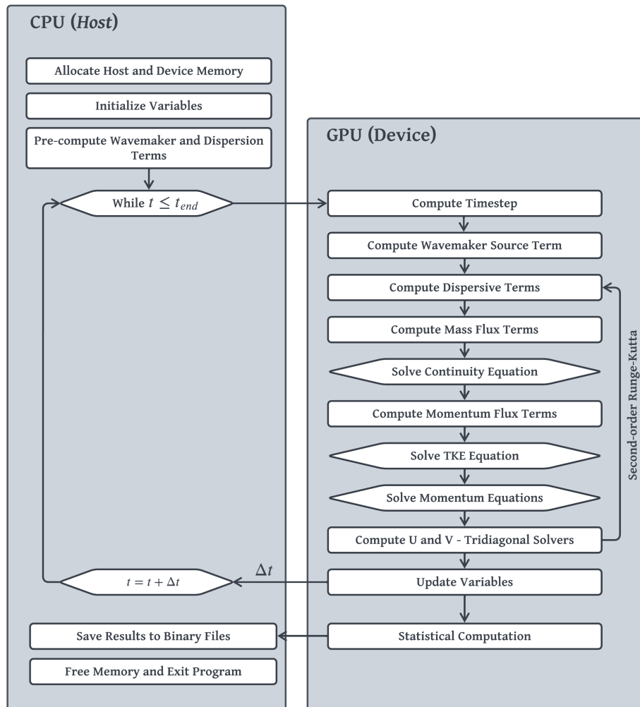
Figure 7.2: GPU Implementation Flow Chart
