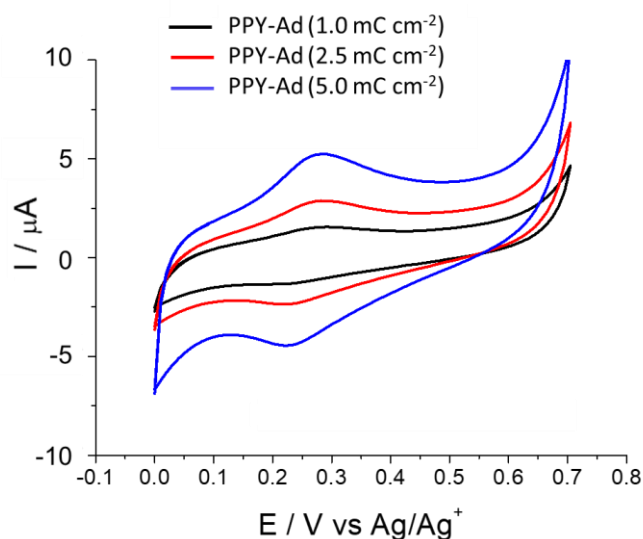
Fig. 6: voltamperograms recorded at Pt electrodes (5 mm diameter disk) after electropolymerization of pyrrole-adamantane ( 3\ mmol\ L^{-1} ) in CH_3CN + LiClO_4\ 0.1\ mol\ L^{-1} at +0.79 V vs Ag/Ag^+ with an electrolysis charge of 1\ mC\ cm^{-2} , 2.5\ mC\ cm^{-2} or 5\ mC\ cm^{-2} and then transferred in CH_3CN + LiClO_4\ 0.1\ mol\ L^{-1} free of monomer.
