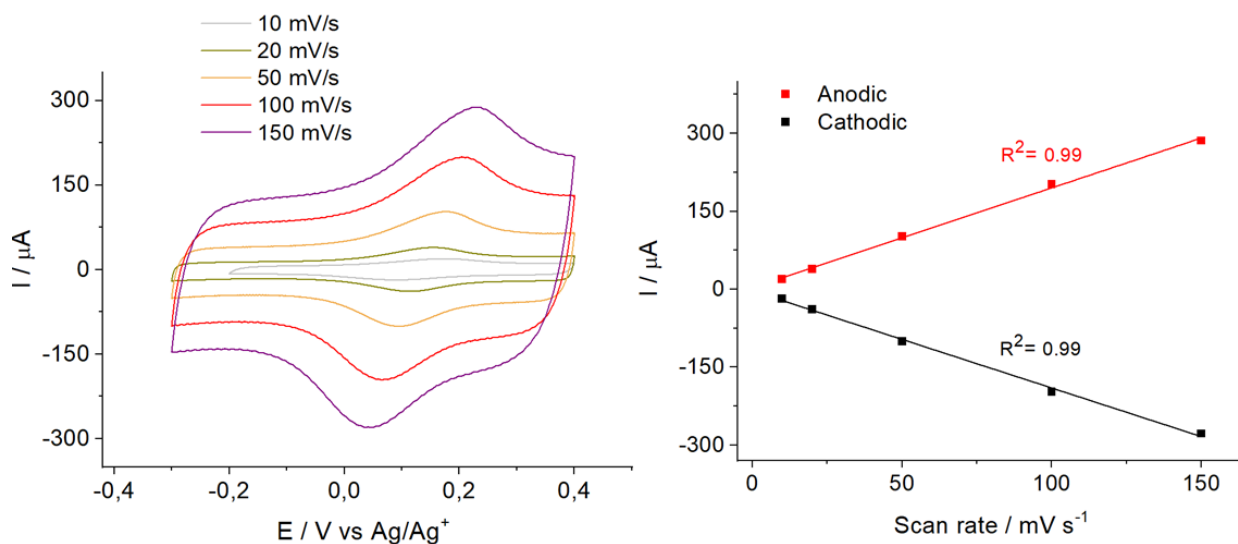
Fig. 14: cyclic voltammograms at variable scan rates of ferrocenyl methanethiol on a functionalized electrode after UV irradiation and the corresponding plot of anodic and cathodic peak currents versus scan rate.
