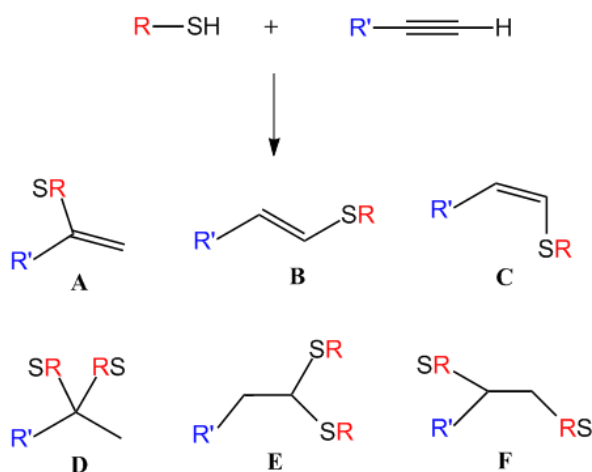
Fig. 1: possible addition products for the mono- and bis-hydrothiolation of a terminal alkyne bond.
