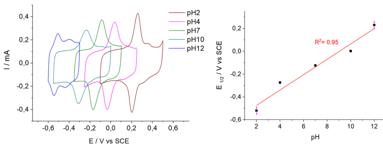
Fig. 30: cyclic voltammograms of one electrode functionalized with 8-mercapto-N-(1,10-phenanthroline-5-yl) octanamide under UV and electro-oxidized in phosphate buffer at pH 2 then cycled again at different pH. Plot of the dependence of the mid point potential versus pH of the electrolytic buffer used. Scan rate: 100 \text{ mV s}^{-1} .
