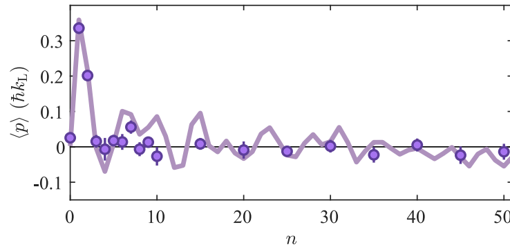
Figure 1.7. Experimental observation of the quantum boomerang effect [21]. In a kicked rotor system, the boomerang effect takes place in momentum space. Time evolution is expressed through the number of kicks n . The results clearly show that, after initial increase of \langle p \rangle , it returns to the initial value. Figure from [21].
