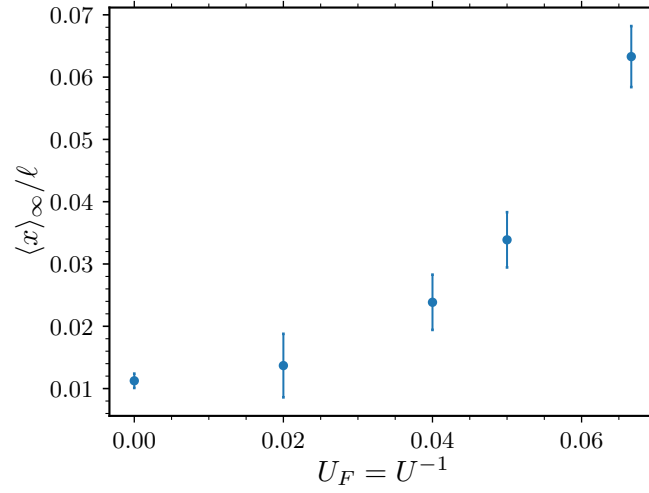
Figure 4.11. Final center of mass position \langle x \rangle_\infty versus U_F = U^{-1} . The errors for the points result from the fitting of the decay Eq. (4.56). Alike in the mean-field study, the dependence of the final CMP on the effective interaction strength between fermions U_F = U^{-1} is quadratic.
