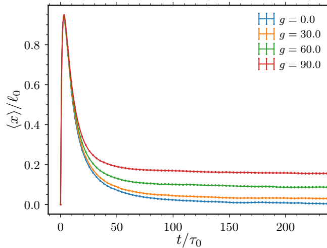
Figure 3.8. Temporal evolution of the center of mass for plane waves calculated using Eq. (3.23) for different values of interaction g . All curves have been averaged over 16000 disorder realizations. The plane wave density is \rho_0 = 1/L = 2.5 \times 10^{-4} k_0 .
