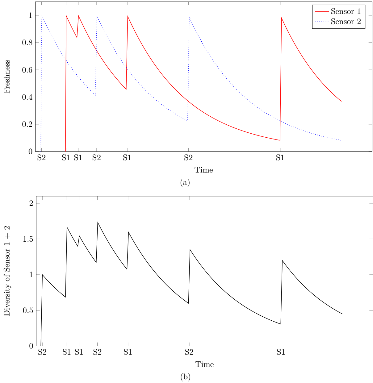
Figure 4.1: Evolution of freshness over time for 2 sensors in (a) and the corresponding diversity in (b). The x-axis represents time, with the observations sent by the sensors labeled as S1 and S2 . The y-axis represents the freshness (or the sum of freshness) according to the observations, with the exponential freshness function.
