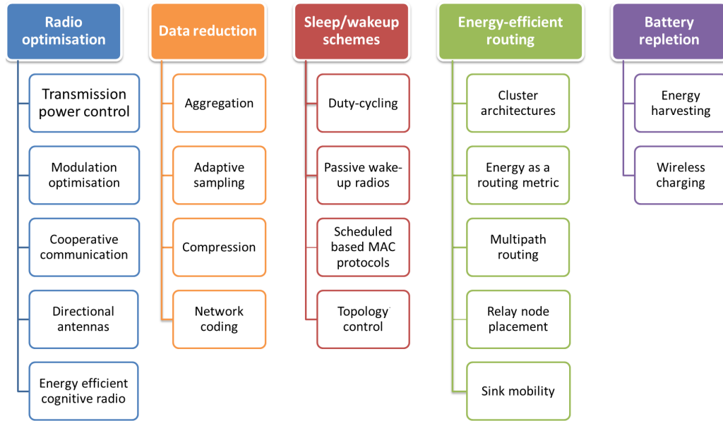
Figure 1.2: Taxonomy of IoT efficient mechanisms, from [RBC14]
