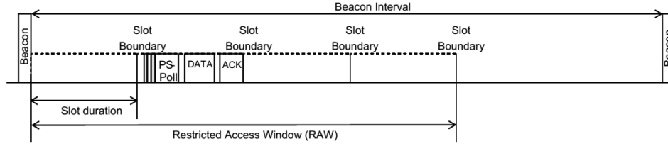
Figure 3.1: A Restricted Access Window (RAW) with CSMA/CA based channel access in a RAW slot [2].
