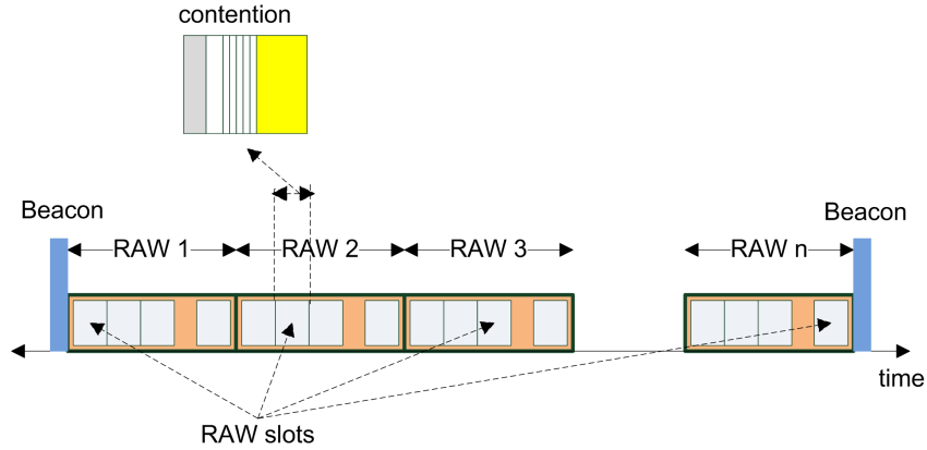
Figure 2.3: Beacon interval representation of the Restricted Access Window MAC approach.
