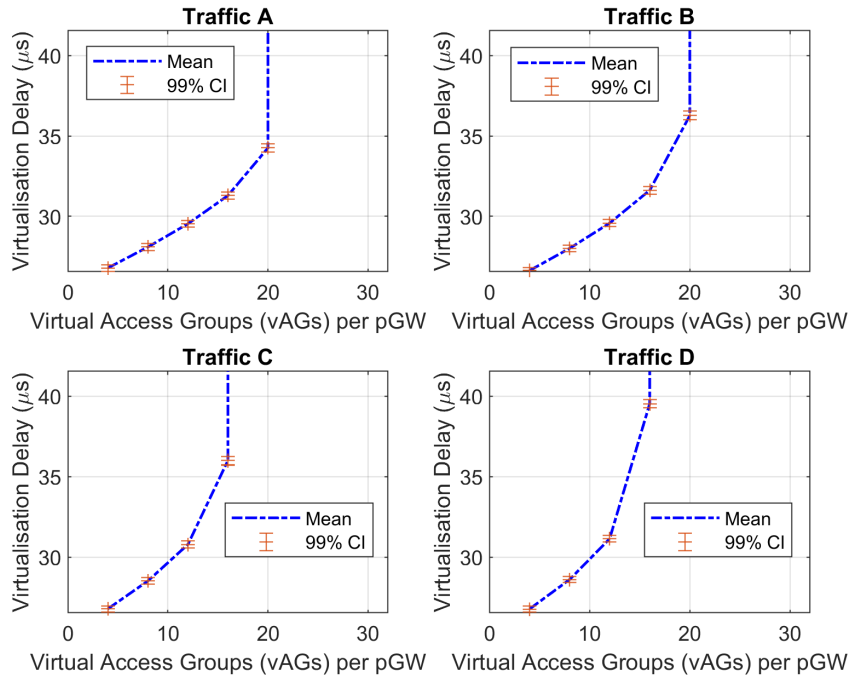
Figure 4.15: Confidence Interval for the simulated (JSIMgraph) virtualisation delay results versus the number of vAGs per pGW node. Confidence level: 99%
