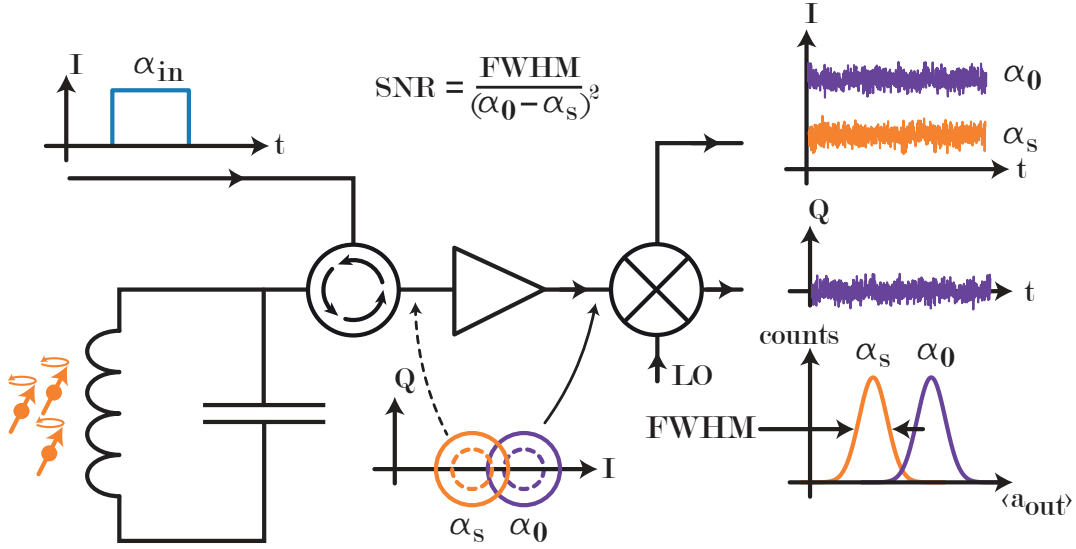
Figure 2.10: Schematic of a continuous wave EPR experiment. The drive of amplitude \alpha_{in} is exciting the spin ensemble. The spin signal \alpha_s leaving the cavity and is amplified together with the bare resonator signal \alpha_0 via a phase-preserving amplifier. Subsequently, the signal is demodulated and detected.
