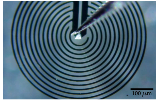
(b) Polypropylene piece being pushed into place using a tungsten tip.
