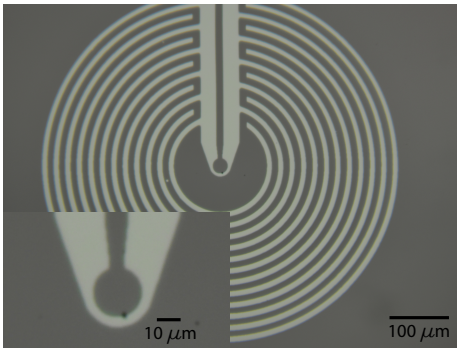
(a) The small black point on the inner loop is a diamond pushed in place.
