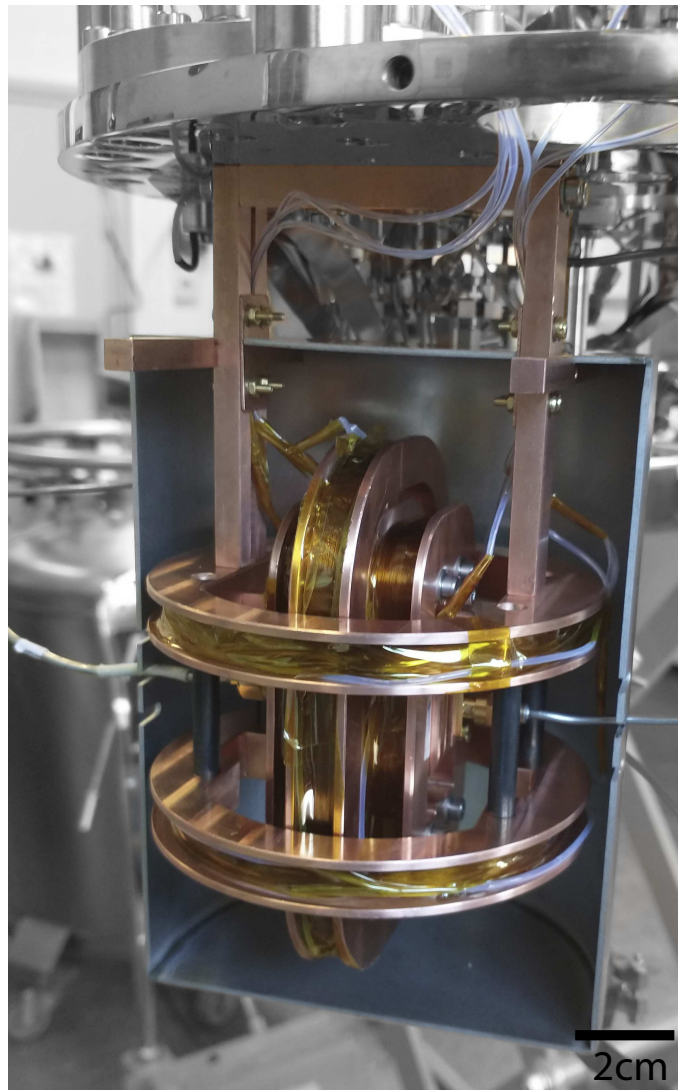
Figure 3.16: The fully assembled magnet including the sample holder is mounted to the 20 mK stage.
