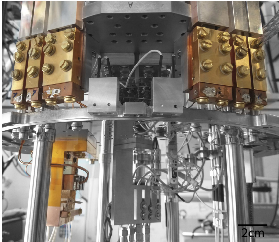
Figure 3.14: Image of the 4 K stage, where the NbTi wires of the magnet are connected with the high T_c wires in the cryostat. The NbTi wires guided through the stage plate within a copper tube leading to the solder connector.
