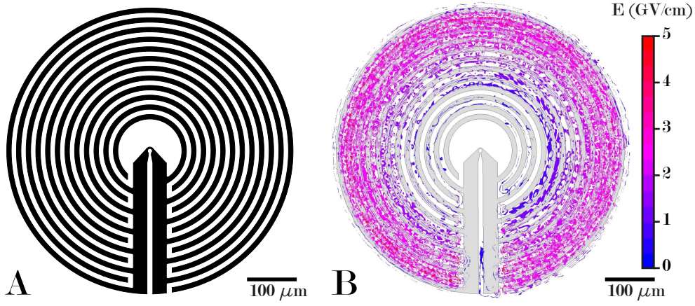
Figure 3.1: A: Example of one resonator using the final design. the sample space is in the centre loop, which in this case has an inner radius of 5 \mu\text{m} . B: Magnitude of the electric field when the resonator is driven on resonance, obtained using a HFSS simulation with 1 W of input power. In the centre of the loop, the electric field is averaged out.
