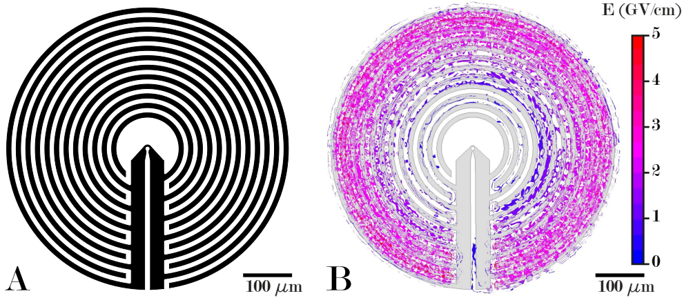
Figure 3.1: A: Example of one resonator using the final design. the sample space is in the centre loop, which in this case has an inner radius of 5\ \mu\text{m} . B: Magnitude of the electric field when the resonator is driven on resonance, obtained using a HFSS simulation with 1 W of input power. In the centre of the loop, the electric field is averaged out.
