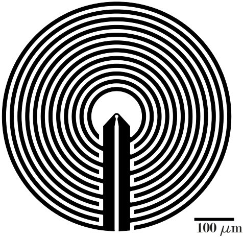
Figure 1.7: Resonator design. The inductive loop in the centre has a radius of 5 \mu\text{m} , the area within this loop is the designated sample space.
