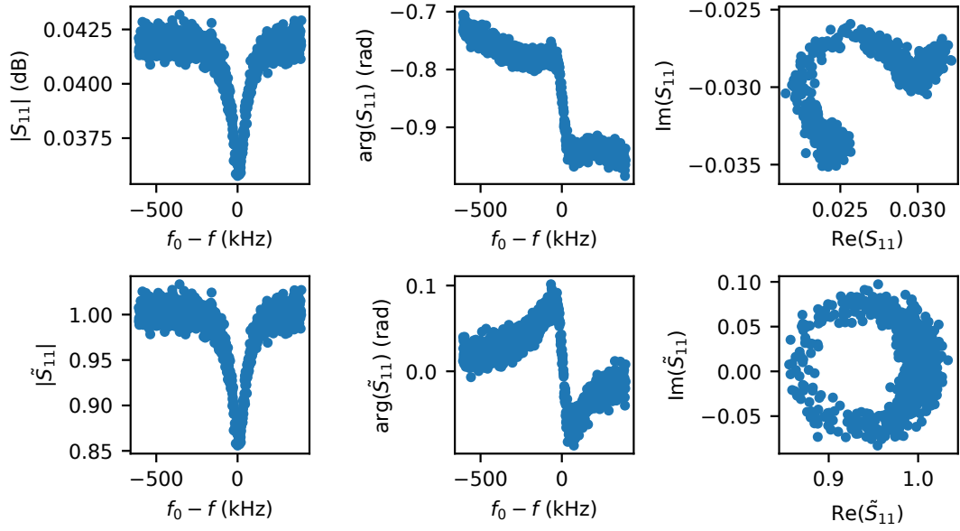
Figure 4.4: Reflection measurement on the BDPA resonator design (resonator 8 on "Sanity TED 90" device). The resonance frequency is f_0 = 7.023\,842 GHz. The upper row shows data without correction of the electric delay. The lower row shows the data after correcting for the electric delay and rescaling by z_\infty .
