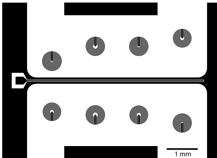
Figure 3.6: Overview of the BDPA design (grey: NbTiN, white: Sapphire). The resonators are labelled 1 – 8 anti-clockwise starting from the lower left.
