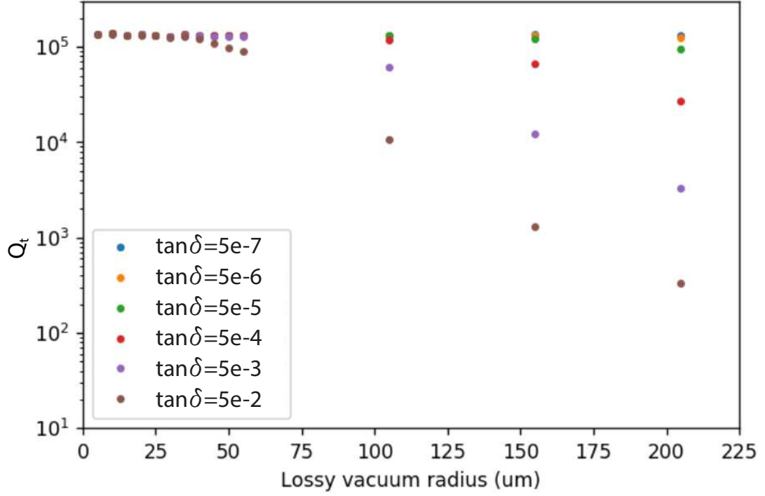
Figure 3.2: Total quality factor versus the radius of a lossy vacuum with height 5\mu\text{m} with different \tan\delta , indicating a resilience of the design for samples with \tan\delta < 5 \cdot 10^{-2} .
