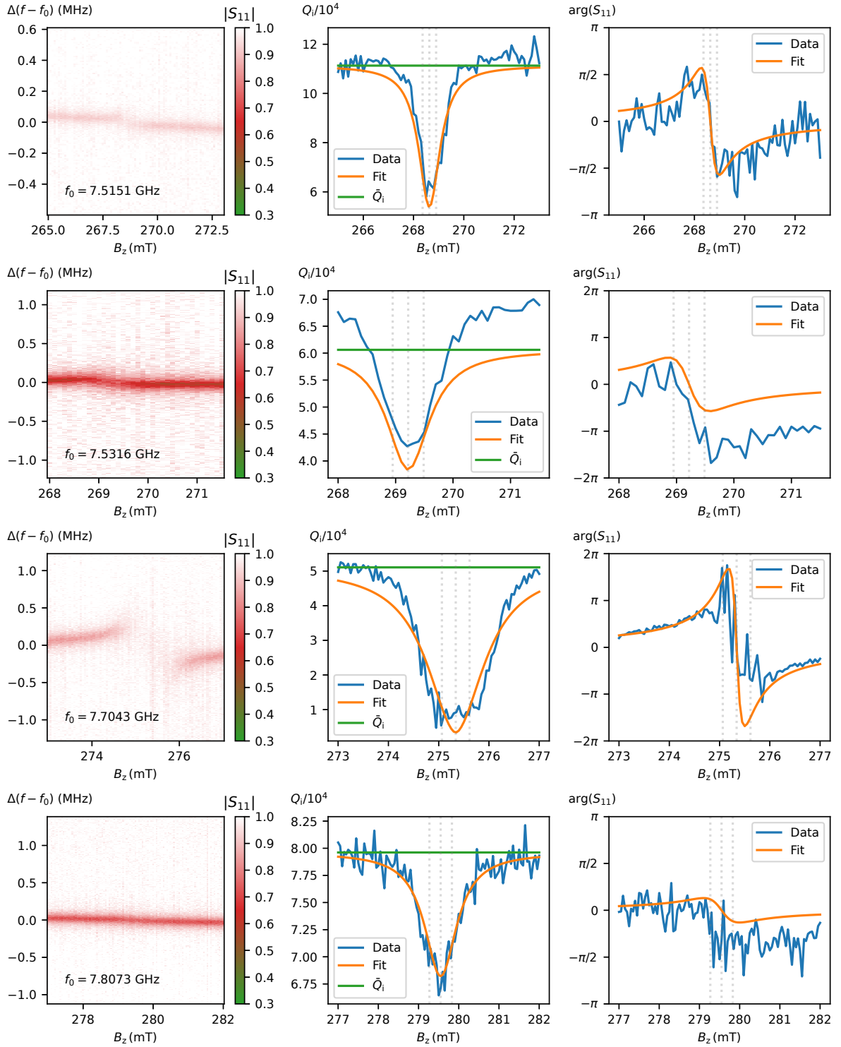
Figure 6.4: Avoided level crossings measured on the resonances (from top to bottom) four to seven. The dotted grey lines indicate the 99.9 % percentiles of magnetic field position. \bar{Q}_i is the average internal quality factor.
