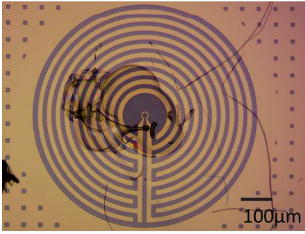
(a) BDPA in PMMA placed manually with a spatula on the circle resonator of the initial device, the capacitate region of the resonator is partially covered.
