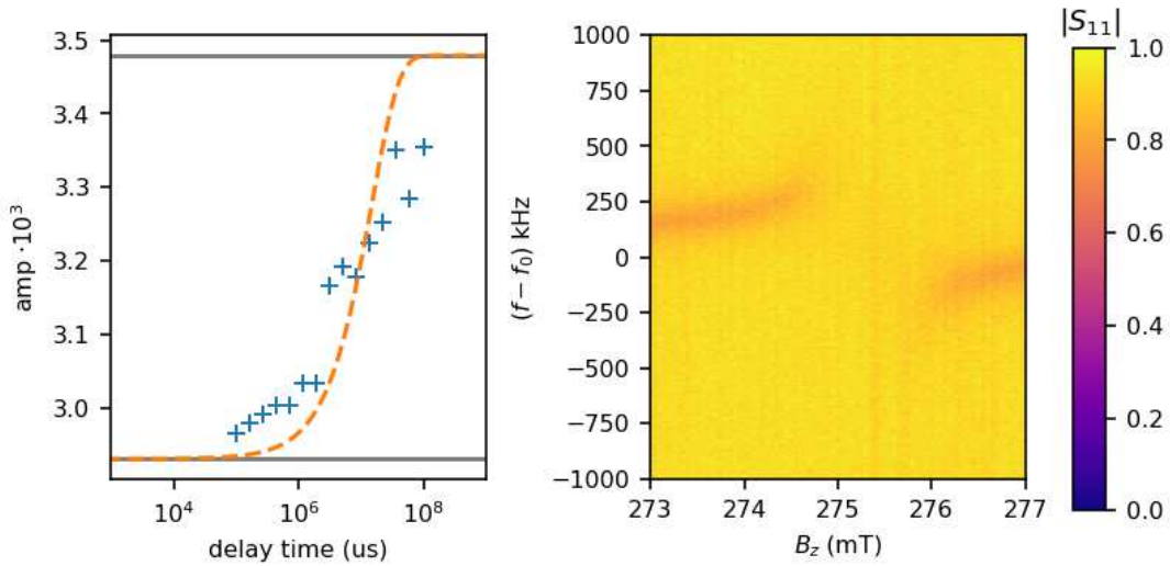
Figure 1.10: T_1 saturation recovery measurement and the avoided level crossing of the measured BDPA. f_0 = 7.70425 GHz.
