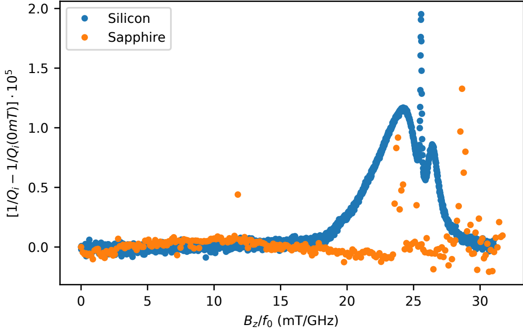
Figure 4.11: Comparison of 1/Q_i - 1/Q_i(0\text{mT}) for the circle resonator of the initial design on sapphire (CHF3 etch, f_0 = 7.89\text{ GHz} ) and silicon (CHF3 etch, f_0 = 6.77\text{ GHz} ). The resonator made on top of silicon displays two broad and one narrow decreases in Q_i , while the losses of the resonator on sapphire are narrow.
