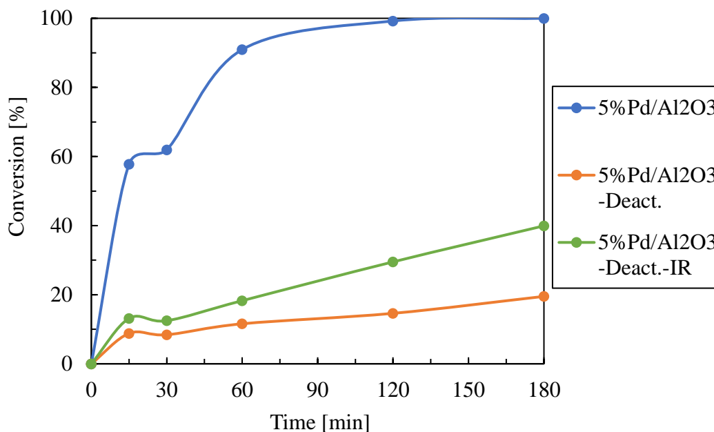
Figure 6-1: Conversion as a function of time of fresh, deactivated and irradiated 5%Pd/Al 2 O 3 catalysts. ( P_{H_2} = 2 \text{ bar} ; T = 60^\circ\text{C} ; M = 2M ; m_{\text{cata}} = 20\text{mg} ; solvent, isopropanol)
