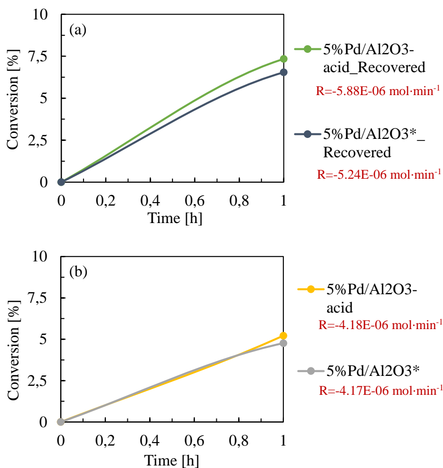
Figure 4-11: Comparison of radioactive and non-radioactive catalyst with (a) Open bottle and (b) Closed bottle. ( P = 0.4 \text{ bar } H_2 ; T = 60^\circ\text{C} ; M = 2\text{M} ; m_{\text{cata}} = 20\text{mg} ; solvent, isopropanol)
