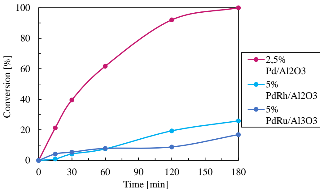
Figure 4-8: Conversion as a function of time for bimetallic catalysts. ( P_{H_2} = 2 \text{ bar} ; T = 60^\circ\text{C} ; M = 2M ; m_{cata} = 20\text{mg} ; solvent, isopropanol)
