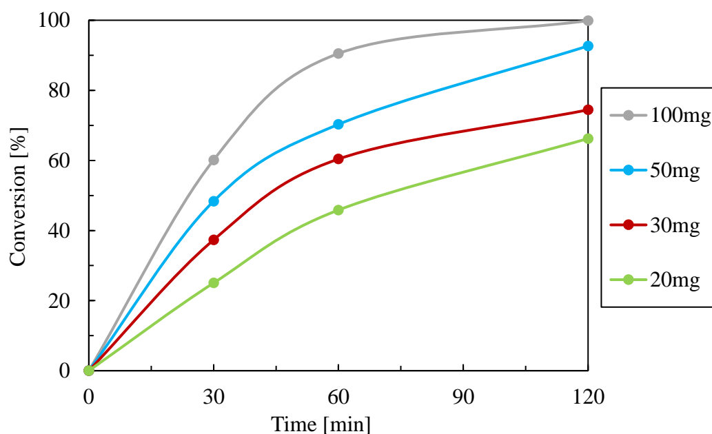
Figure 4-4: Evolution of CNA conversion as a function of time for different amounts of catalyst mass. ( P_{H_2} = 2 \text{ bar} ; T = 60^\circ \text{C} ; M = 2 \text{ M} ; solvent, isopropanol 5%Tri/Al 2 O 3 )
