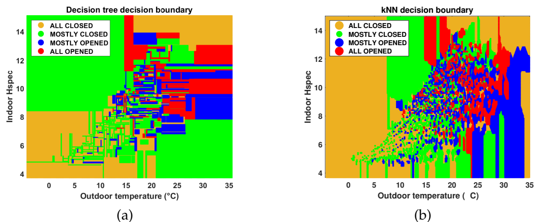
Figure 8.8: Decision boundary for a window status prediction model based on outdoor temperature and indoor specific humidity when using (a) Decision Tree model or (b) k-NN model.
