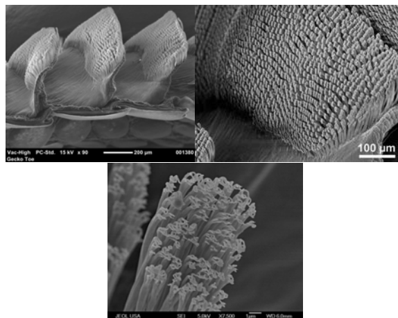
Fig. I.3 From left to right: the lamellae under each toe of a gecko's paw, the array of setae , the spatulae at the end of each seta . Images available at https://geckskin.umass.edu/images for educational and non-commercial use only
