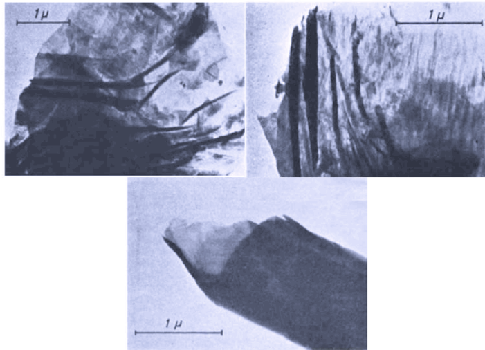
Fig. 3.21 Three pictures from the original article written in 1960 by Bollmann and Spreadborough, Action of Graphite as a Lubricant . Top left: a complex system of rollers. The picture is magnified \times 15,000 . Top right: parallel carbon whiskers close to the edge of a crystal. Bottom: a detail of a single carbon structure. These last two pictures are magnified \times 24,000 . Source: Bollmann and Spreadborough (1960)
