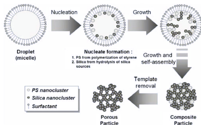
Fig 5.10 The necessary steps to prepare mesoporous silica nanoparticles. Source: Nandiyanto, Kim, Iskandar and Okuyama (2009)
