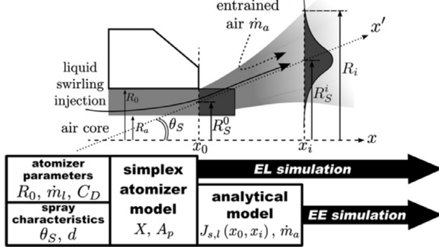
Figure 3.4: FIMUR model for injection in pressure-swirl atomizers. Source: Sanjose et al. (2011).
