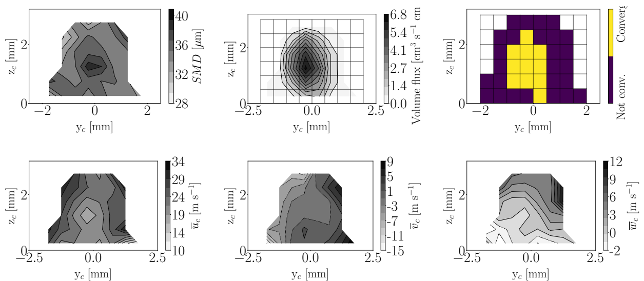
Figure 8.33: Spray states at x_c = 2 mm for case DX10
