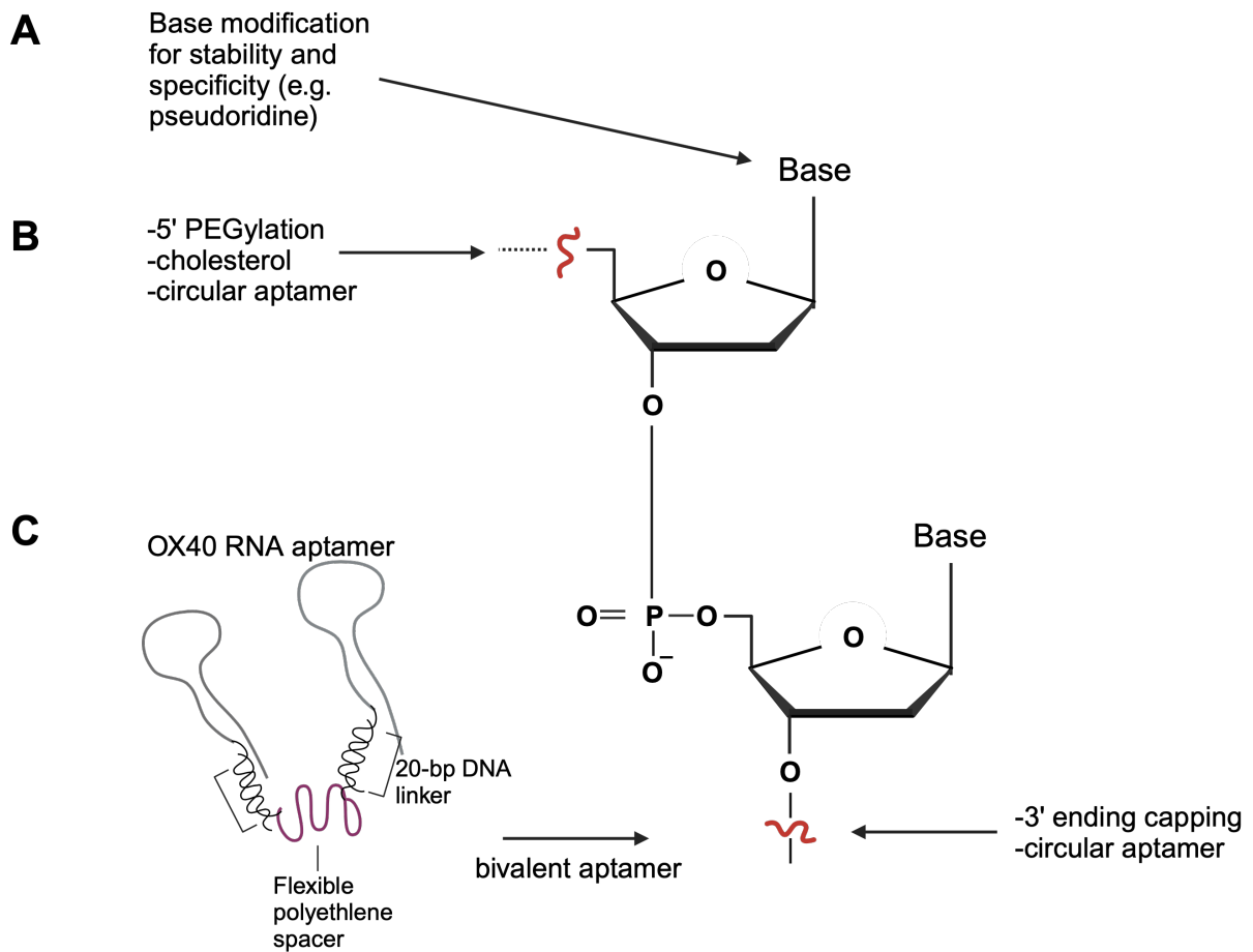
Figure 35: Strategies used to increase the stability and/or specificity of an aptamer.
