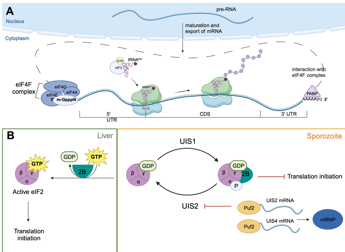
Figure 10: Overview of translation initiation and its control in the pre-erythrocytic stage.
