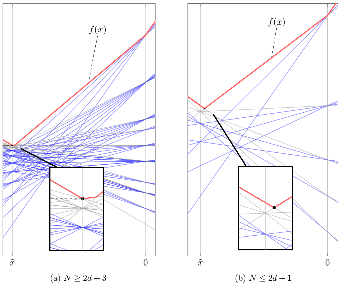
Figure 10 – The optimal value of the dual optimization problem lies at the intersection of the set of affine functions f_{\lambda,\mu}(x) . When N \geq 2d + 3 (Figure 10a, with N = 9 and d = 3 ), then p^*(N, d) = g(\lambda_1) . When N \leq 2d + 1 (Figure 10b, with N = 5 and d = 3 ), then p^*(N, d) lies at the intersection of f_{\lambda_2,\mu_1} and f_{\lambda_1,\mu_2} . In ■ the max over all affine functions, in ■ the affine functions from the set \Gamma , and in ■ the affine functions from the set \Omega \setminus \Gamma .
