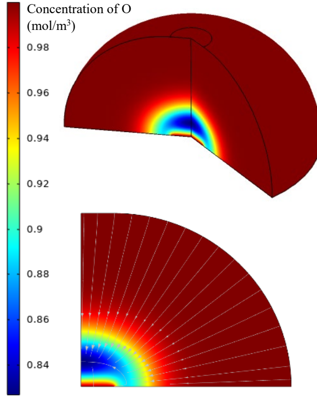
Figure 4.4: Concentration profile at t = 20 s, E⁰ = 0 V on 2D axisymmetric and 3D simulations
