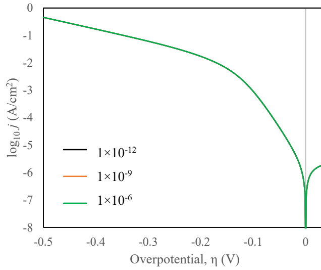
Figure 6.14: Tafel plots for 3D simulation (no kinetic parameters permutation) with edge effect and surface diffusion, D_{surf} = 1 \times 10^{-12}, 1 \times 10^{-9}, 1 \times 10^{-6} \text{ m}^2/\text{s} .
