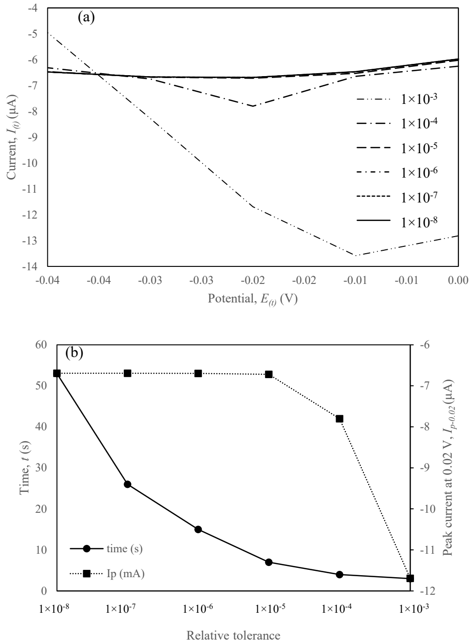
Figure 4.11: (a) Plot of relative tolerance ( rtol ) for current, I(t) vs potential, E(t) and (b) Computation time, t in s, and peak current value at -0.02 V, I_{p-0.02} in \mu\text{A} vs relative tolerance ( rtol ) for 1-D model
