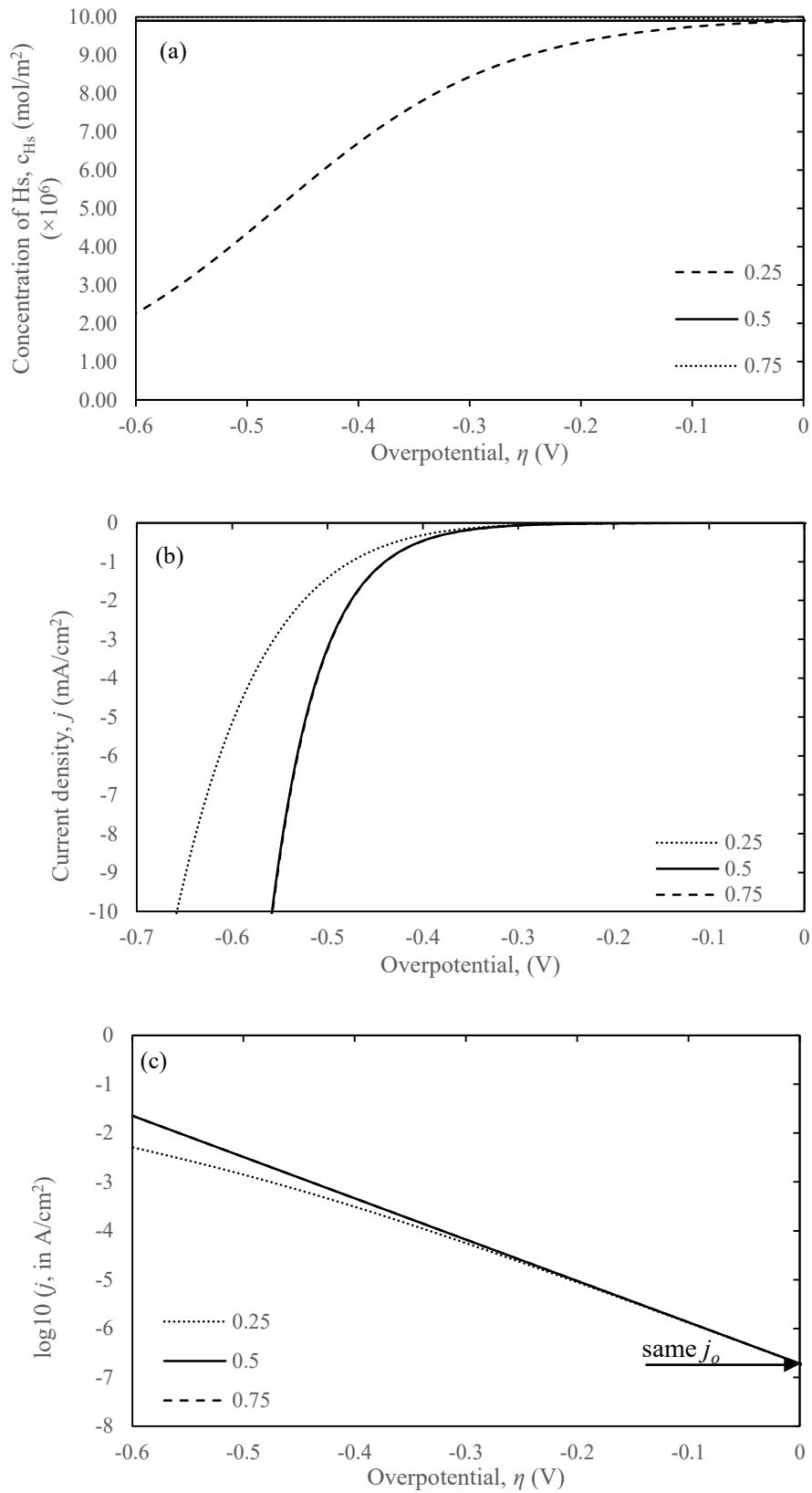
Figure 5.3: Comparison on the Volmer charge transfer coefficient, \beta_v = (0.25, 0.5, 0.75) against overpotential, \eta , on the (a) concentration profile of H_s , c_{Hs} (mol/m 2 ) (b) current density, j (mA/cm 2 ) and (c) the corresponding Tafel plots in A/cm 2 .
