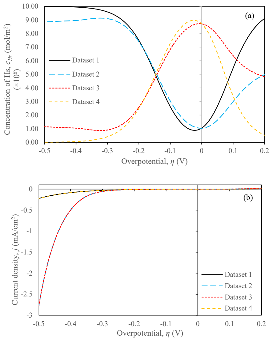
Figure 6.6: Corresponding (a) c_{H_s} (mol/m 2 ) vs \eta (V) and (b) the j (mA/cm 2 ) vs \eta (V) for TiC and taC:Pt from Tafel plots Figure 6.5.
