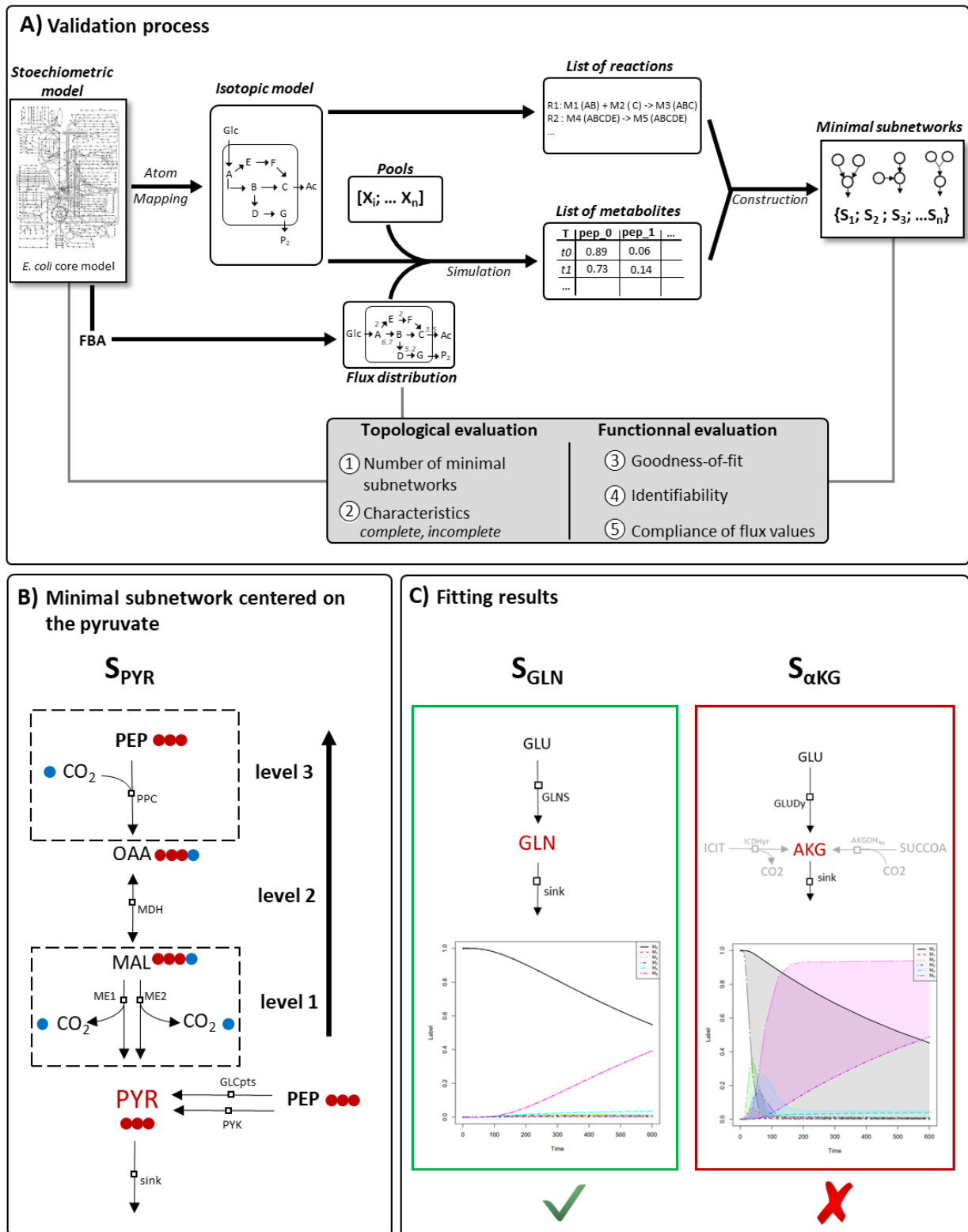
Figure 3.4 : Validation of the Network Analyzer. A. Validation process. The Network Analyzer is validated using a GSM and a theoretical dataset based on topological and fonctionnal criteria. B. Minimal subnetwork centered on the pyruvate. The elementary metabolite unit producing the three atoms of carbon of the pyruvate is retrieve at the third level of extension. The final LLI of the pyruvate is the phosphoenolpyruvate. C. Fitting results of two minimal subnetworks ( S_{GLN} and S_{\alpha-KG} ). The reactions that were not conserved during the construction process are in grey.
