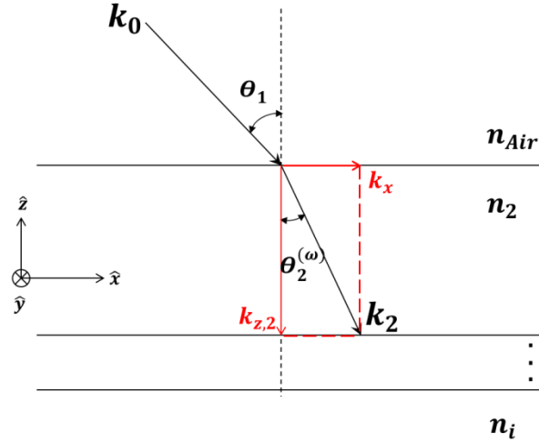
Figure 3.3: Geometry for the propagating fundamental fields between the air and medium “ i ”, presenting the angle of incidence, the refraction angle and the wavevectors with the projection on x - and z -axis. Note that the refractive index n_i in this schematic is assumed to be real.
