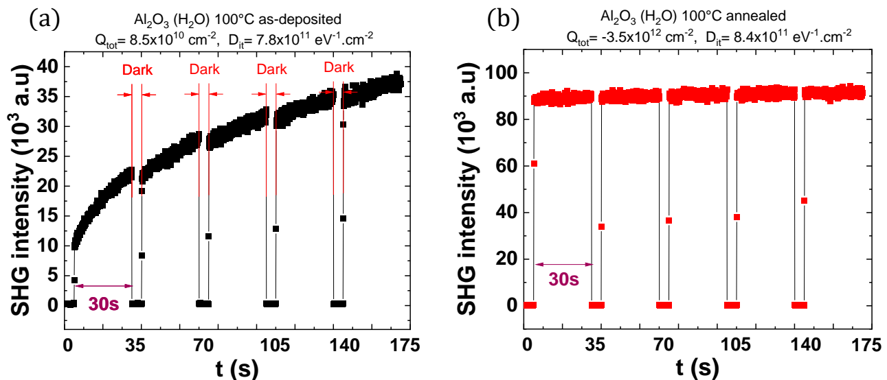
Figure 5.6: Five consecutive TD-SHG measurements at the same spot on the sample Al 2 O 3 (H 2 O) 100°C on Si, (a) before and (b) after annealing the wafer.
