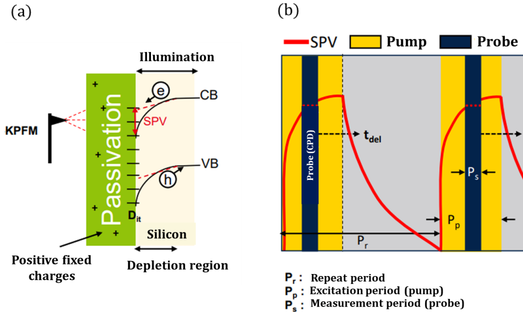
Figure 1.15: (a) KPFM measurement principle. (b) pp-KPFM approach. Figures taken from [33].
