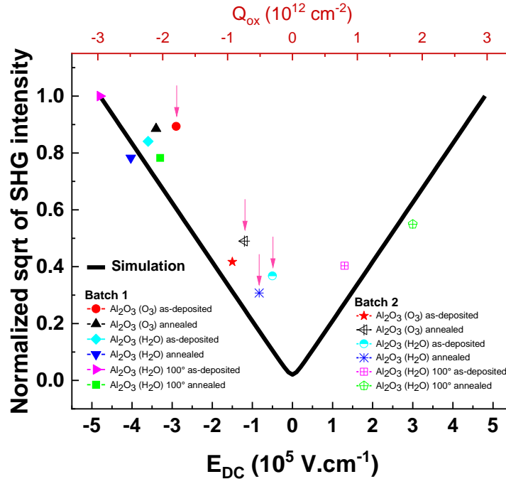
Figure 5.16: Simulated and experimental SHG versus E_{DC} (bottom axis) and Q_{ox} (top axis) from all the Al_2O_3 samples. The experimental E_{DC} values were calculated using C-V results presented in Table 5.3.
