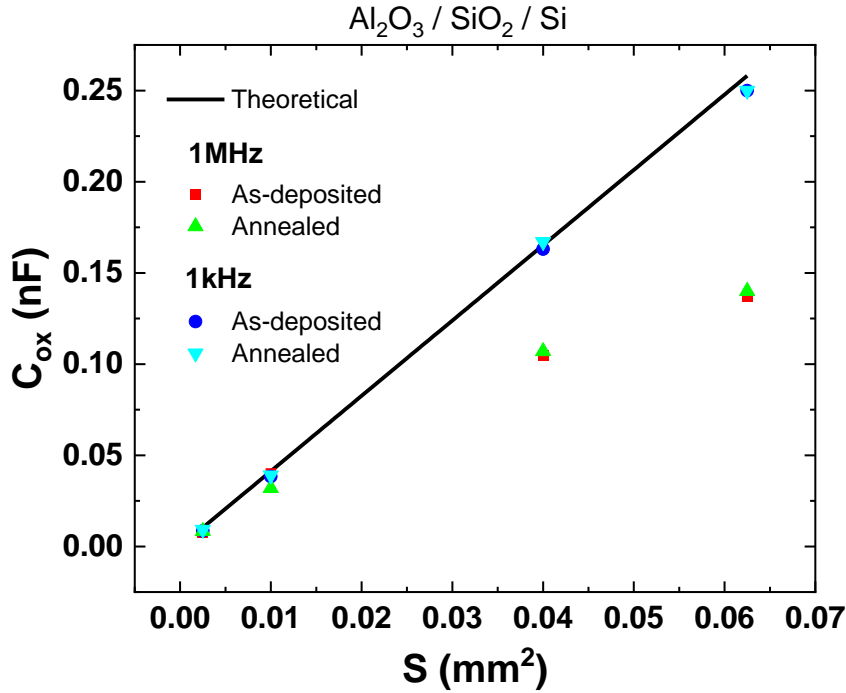
Figure 4.11: Capacitance versus MOS surface area for \text{Al}_2\text{O}_3/\text{SiO}_2/\text{Si} sample.
