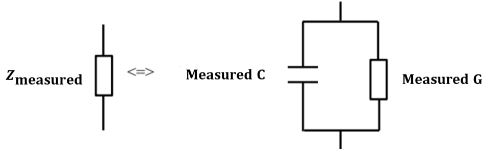
Figure 1.10: Equivalent circuit of MOS structure for capacitance and conductance measurements. Figure taken from [9].
