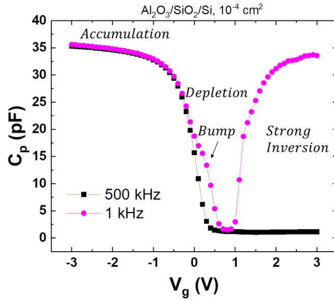
Figure 4.10: C-V curves measured from Al 2 O 3 /SiO 2 /p-type Si sample at low and high frequencies.
