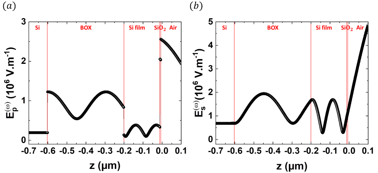
Figure 3.6: Variation of fundamental electric field in z -axis direction in SOI structure (Si substrate/ 0.4 \mu\text{m} BOX/ 0.19 \mu\text{m} Si film) with native oxide for the case of (a) P_{in} polarization and (b) S_{in} polarization.
