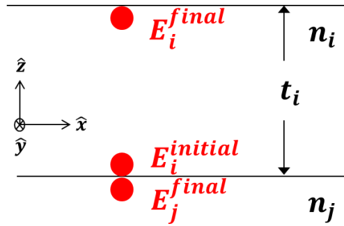
Figure 3.4: The electric fields propagation between and within the layers of multilayer structure [14].
