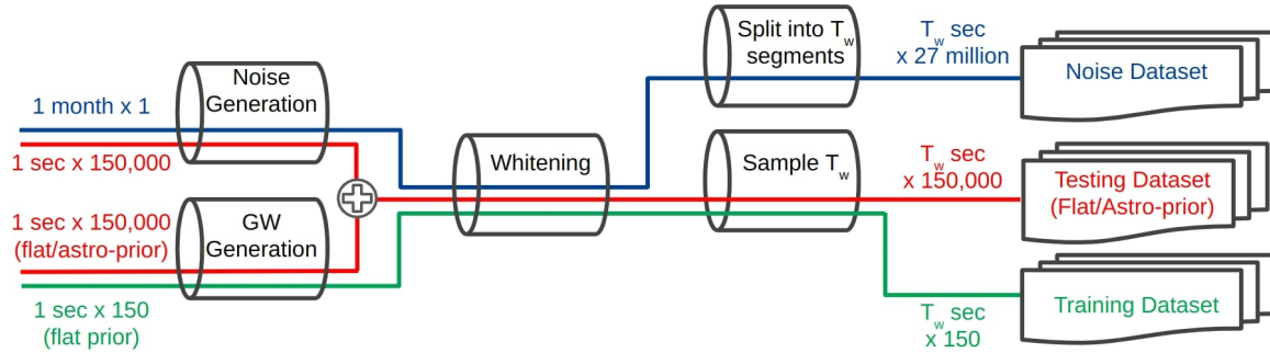
Figure 4.3: Flowchart illustrating the procedures involved in generating the noise, training, and testing datasets. The size of the data are written in text in the format duration of each realization \times number of such realizations .
