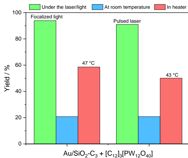
Figure 31. Results for cyclooctene oxidation over Au/SiO 2 -C 3 + [C 12 ] 3 [PW 12 O 40 ] NPs under light or laser irradiation, room temperature and external heating. Reactions conditions: 30 mg Au/SiO 2 -C 3 NPs, 50 mg [C 12 ] 3 [PW 12 O 40 ] NPs, 1.5 mL toluene (containing 2 mol/L cyclooctene) and 1.5 mL water (containing 1.2 equiv. H 2 O 2 ), emulsification at 11,500 rpm for 2 min, 120 rpm, 60 min, 120 rpm. Results based on 1 H NMR.
