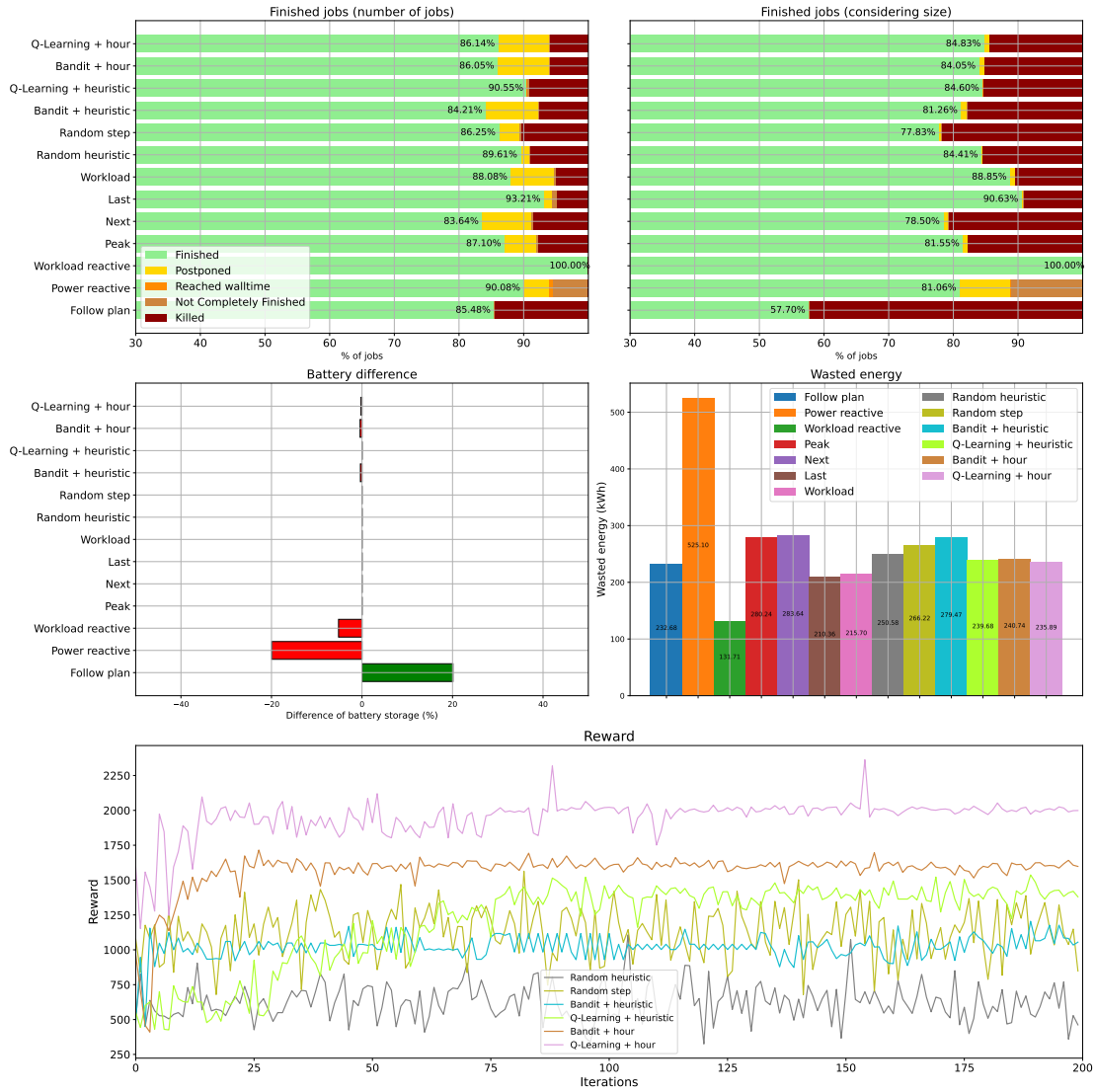
Figure 5.3: Results of Started Jobs Reward in critical case 2.
