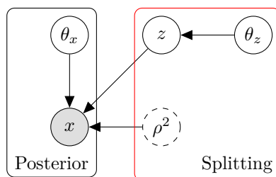
Figure 5.1: DAGs associated with the proposed hierarchical Bayesian model. In black: DAG associated to (5.6) and in red: DAG associated to (5.7). \theta_z stand for that parameters of the deep learning based prior model and \theta_x for possible additional parameters of the forward model.
