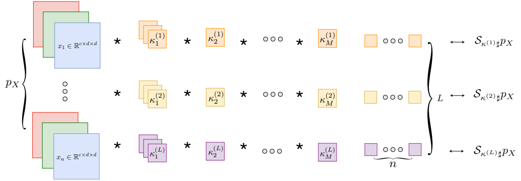
Figure 2.2: The convolution slicing process. The images are directly mapped to a scalar by a sequence of convolution functions which have kernels as random tensors
