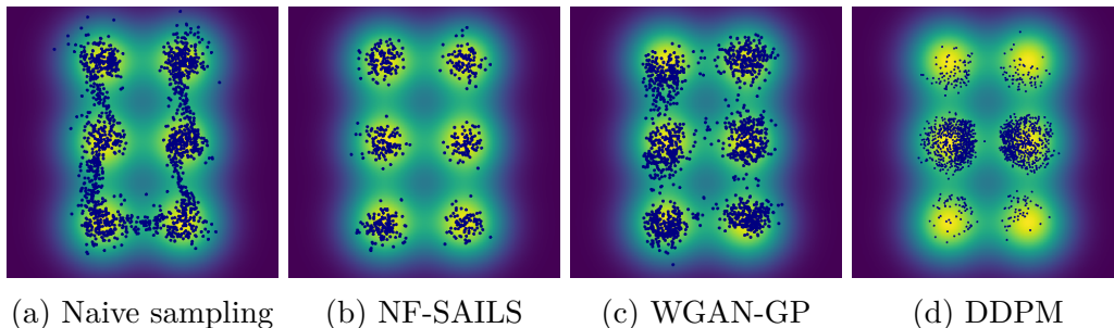
Figure 4.3: Mixture of k = 6 Gaussian distributions (green), and 1000 generated samples (blue). The proposed NF-SAILS method in Fig. 4.3b does not generate samples in-between modes.
