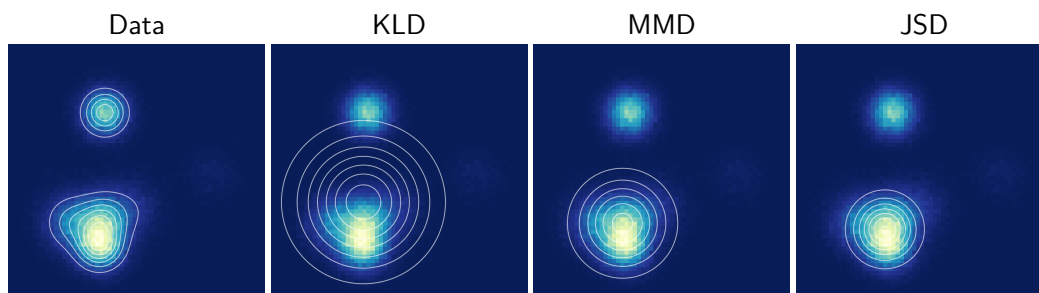
Figure 1.4: An isotropic Gaussian distribution was fit to data drawn from a mixture of Gaussians. Training procedure from left to right: minimizing Kullback-Leibler divergence (KLD), MMD, JSD. The different fits demonstrate different tradeoffs made by the three divergences. Results reported in [31].
