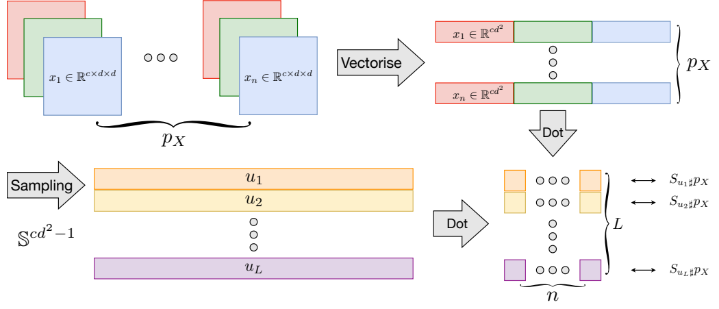
Figure 2.1: The conventional slicing process of sliced Wasserstein distance.
