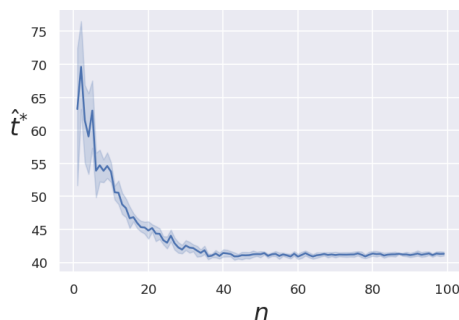
Figure 5.5: Inpainting: evolution of \hat{t}^* along the PnP-SGS iterations ( T = 1000 ). Results have been averaged over 100 runs conducted on the same image. Shaded areas stand for the corresponding standard deviation.
