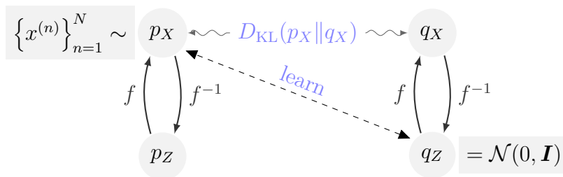
Figure 4.2: NF learns a mapping f from data points \{x^{(n)}\}_{n=1}^N assumed to be drawn from p_X towards the latent Gaussian measure q_Z . The training consists in minimizing the KL divergence between p_X and q_X = f_{\#}q_Z . Once trained, the learnt map permits to go from q_Z to q_X , which is an approximation of the true target distribution p_X .
