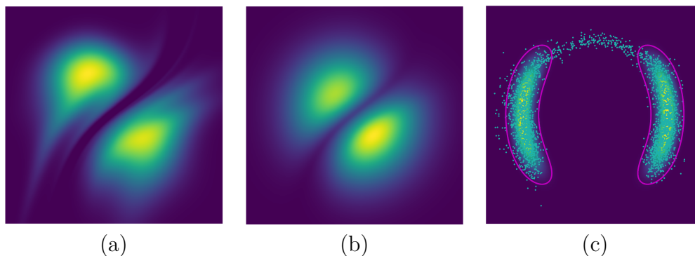
Figure 4.1: (a) Target distribution p_Z in the latent space; (b) Learnt latent distribution in the latent space q_Z ; (c) Output of naive sampling, i.e., \{x^{(n)}\}_{n=1}^N with x^{(n)} = f(z^{(n)}) and z \sim q_Z .
