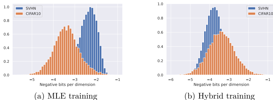
Figure 2.5: Likelihood histogram for 1000 CIFAR-10 images (orange) and 1000 SVHN images (blue) prescribed by a CSW-NF trained on CIFAR-10 images.
