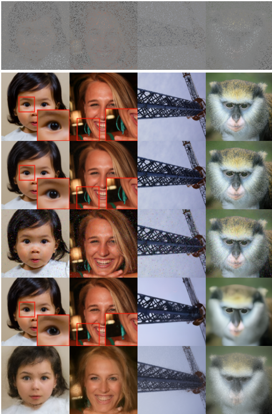
Figure 5.2: Inpainting task on the FFHQ (first two columns) and Imagenet data sets (last two columns), from up to bottom: measurement, true image, PnP-SGS ( \mathbf{x}_{\text{MMSE}} ), SPA [137], MCG [159], DDRM [158].
