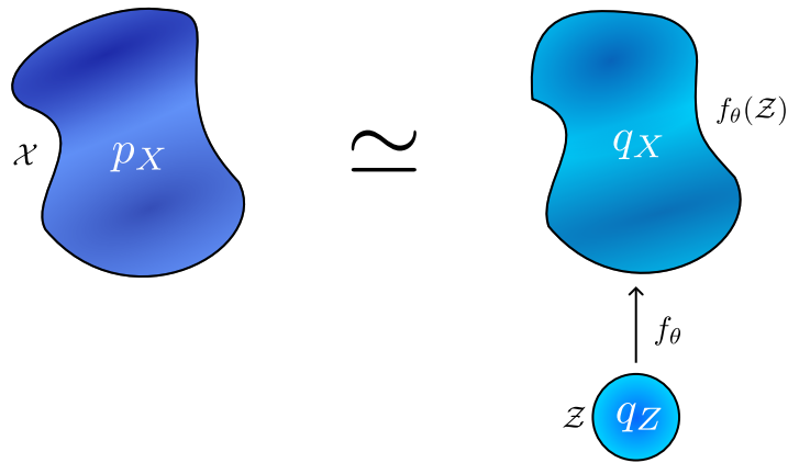
Figure 1.3: The deep generative model f_\theta aims at mapping samples from a simple distribution q_Z (located at the bottom right) to a more complex distribution q_X (located at the top right), with the objective of achieving similarity to the true distribution p_X (located at the top left).
