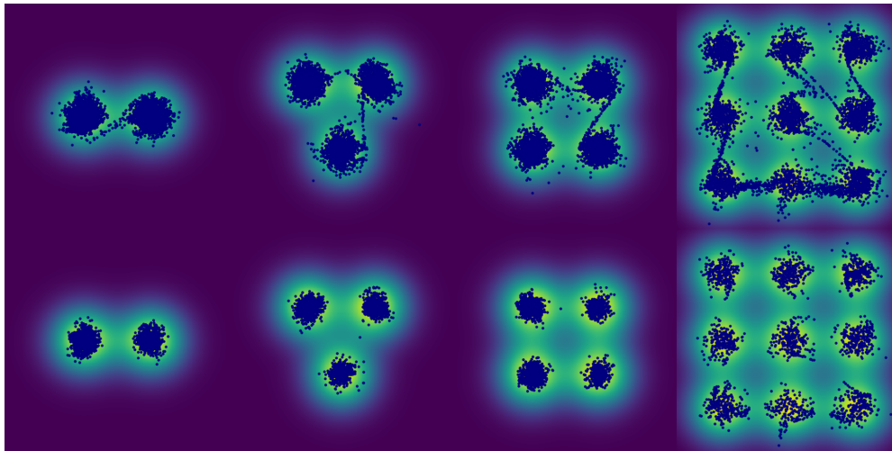
Figure 4.4: Mixture of k Gaussian distributions (green), and 1000 samples (blue) generated by the naive sampling (top) and the proposed NF-SAILS method (bottom) with, from left to right, k = 2 , k = 3 , k = 4 and k = 9 .
