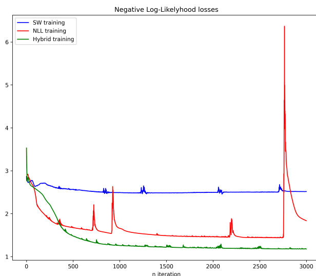
Figure 2.4: Evolution of the negative log likelihood prescribed by the model during training. In blue SW training, in red MLE training, in green hybrid training.
