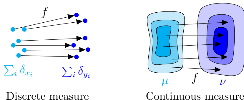
Figure 3.1: Comparison of the push-forward operator f_# , which can take as an input any measure
