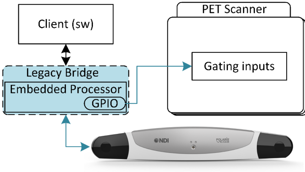
Figure 3.4 Legacy-mode connection scheme with available PET gating input.
