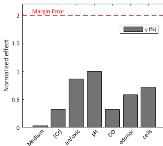
Figure II.17. Effect of each factor for response variable \eta_{Cr} . Values are normalized by the most significant effect, in this case is the pH.
