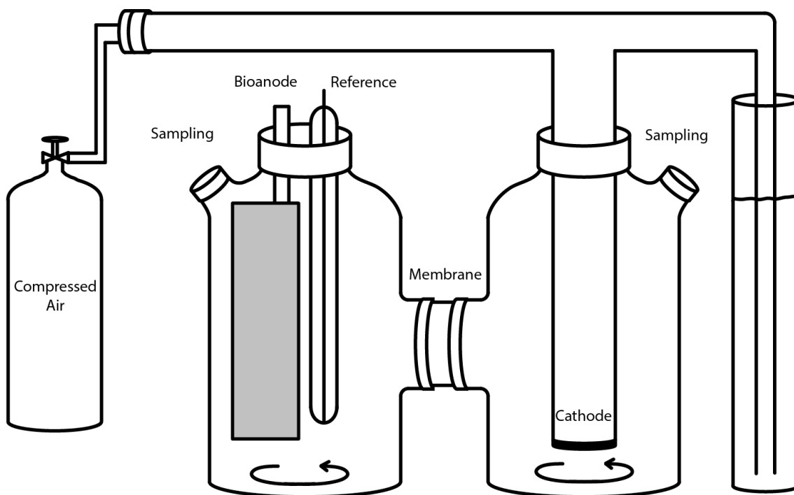
Figure III.7. BES/GDE set-up.
