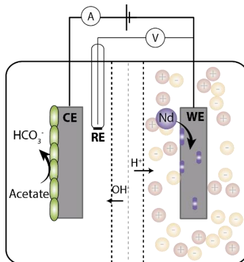
Figure IV.6. Microbial Electrochemical System for Nd electrodeposition with an IL catholyte.
