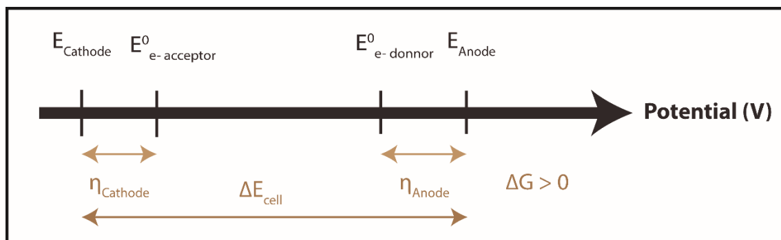
Figure I.12. Schema of redox potentials in a MEC.
