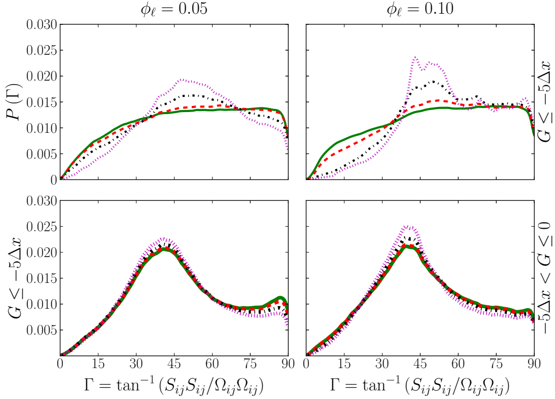
Figure 5.17. PDF of the strain-entropy angle \Gamma conditioned for four threshold values : 0.25\|\mathbf{g}^{\tilde{\zeta}}\| (—), 0.5\|\mathbf{g}^{\tilde{\zeta}}\| (- - -), 1.0\|\mathbf{g}^{\tilde{\zeta}}\| (- · - ·), and 1.5\|\mathbf{g}^{\tilde{\zeta}}\| (· · · ·); in the G \leq -5\Delta x (far+intermediate, top), and near (bottom) regions from the liquid-gas interface for \phi_\ell = 0.05 (left) and \phi_\ell = 0.10 (right).
