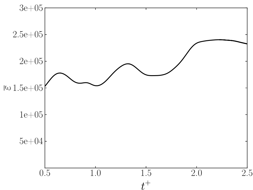
Figure 3.4. Evolution of the mean dissipation rate of the turbulent kinetic energy, \bar{\epsilon} (—), as function of the non-dimensionalized time, t^+ , for the HIT reference case.
