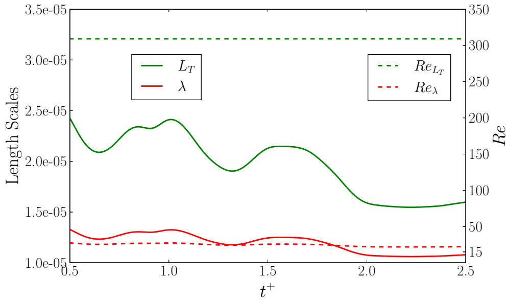
Figure 3.5. Evolution of the integral, \ell_t (—), and Taylor, \lambda (—), length scales; together with their corresponding turbulent, Re_{\ell_t} (---), and Taylor, Re_\lambda (---), Reynolds numbers, as a function of the non-dimensionalized time, t^+ , for the HIT reference case.
