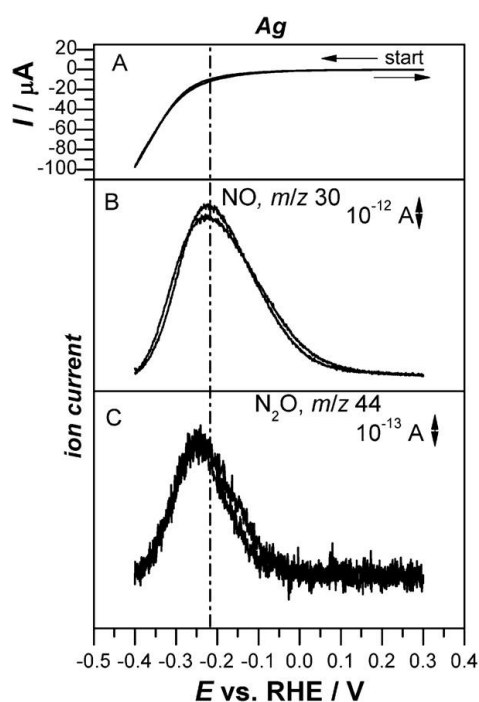
Figure 3.3.1 Cyclic voltammetry during OLEMS measurements (A) and ion current profiles for m/z = 30 (B) and m/z = 44 (C) in 0.1 M HClO_4 containing 1.6 mM NaNO_2 . The working electrode is a polycrystalline Ag bead electrode, v = 1 \text{ mVs}^{-1} . The dashed dotted line indicates the onset potential for hydrogen evolution. The arrows indicate the direction of the potential sweep. 1d
