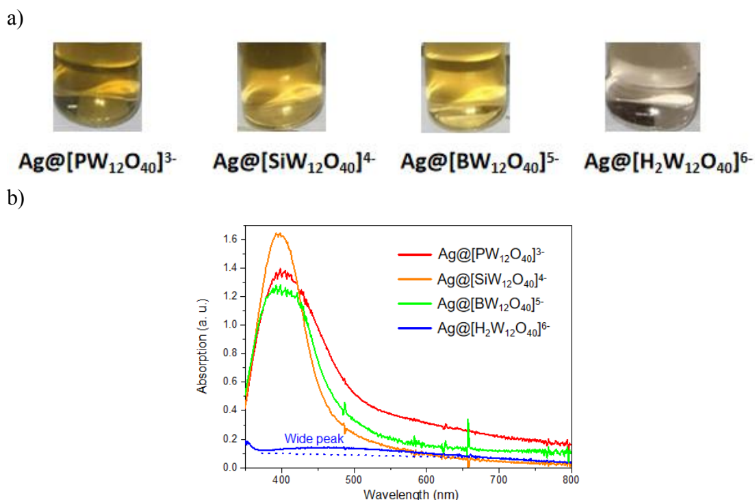
Figure 3.4.5 a) Picture of four solutions containing Ag@POM NPs. B) UV-Vis spectra of solution in a).
