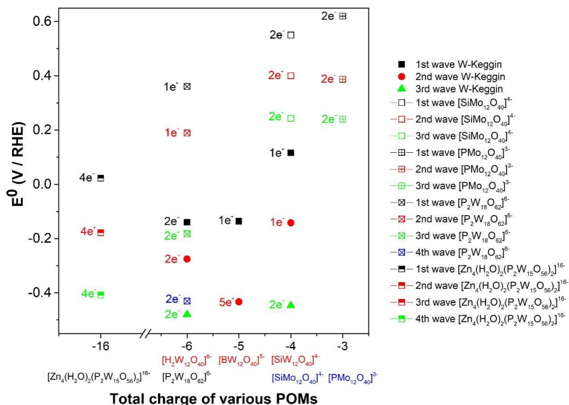
Figure 2.2.9 Comparisons of formal potential of all POMs studied in this work, at pH 2. Only [\text{PW}_{12}\text{O}_{40}]^{3-} is missing due to its instability at \text{pH} > 1.7 .
