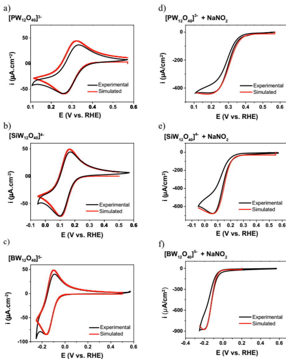
Figure 2.7.1 Comparison of experimental data of cyclic voltammery (black curves) and simulated curve with the microkinetic model (red curves) for three POMs at pH 1 in the absence of nitrite (a-c) and in the presence of 10 mM of NaNO_2 (d-f). Experimental conditions: scan rate, 20\text{ mVs}^{-1} ; 1 mM POM; electrolyte: 0.5 M Na_2SO_4 + H_2SO_4 , pH 1.
