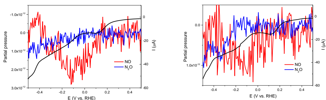
Figure 3.4.12 DEMS study of nitrite reduction at pH 2 catalyzed by: a) [\text{SiW}_{12}\text{O}_{40}]^{4-} at GC electrode; b) \text{Ag@[SiW}_{12}\text{O}_{40}]^{4-} at GC electrode. Black curve: the forward scan of cyclic voltammetry ( 0.5 \text{ mVs}^{-1} ); Red curve: the signal of m/z 31 ( ^{15}\text{NO} ); Blue curve: the signal of m/z 46 ( ^{15}\text{N}_2\text{O} ). Experimental conditions: a) 0.1 mM [\text{SiW}_{12}\text{O}_{40}]^{4-} and 0.1 M 2-propanol; b) 0.02 mM of \text{Ag@[SiW}_{12}\text{O}_{40}]^{4-} , 0.1 mM [\text{SiW}_{12}\text{O}_{40}]^{4-} , and 0.1 M 2-propanol. For both a) and b) 10 mM \text{Na}^{15}\text{NO}_2 and pH 2, 0.5 M \text{Na}_2\text{SO}_4 .
