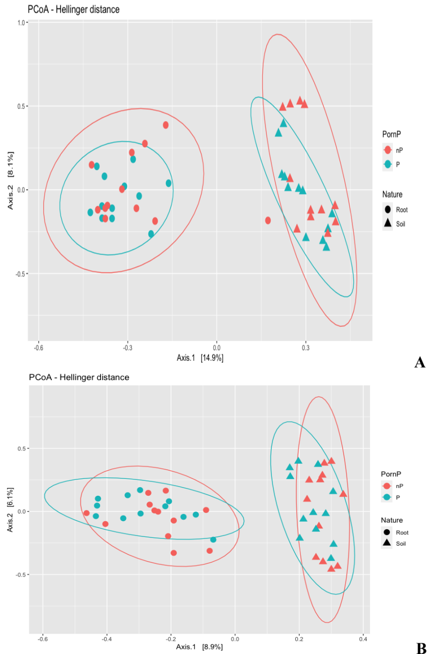
Figure 3: Beta-diversity analysis among the over-all data set: PCoA ordination, based on Hellinger distances, of bacterial 16S rRNA gene sequence data (A) with p value=0.024 and fungal ITS sequence data (B) with p value=0.0168.
