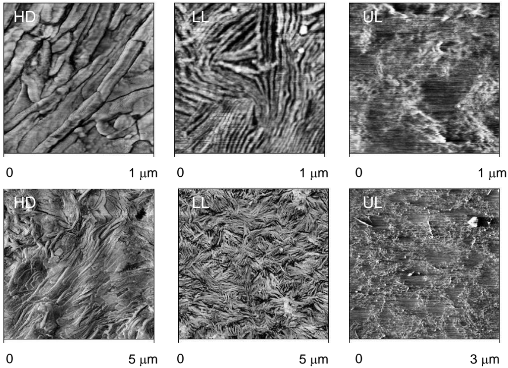
Fig. IV.3. AFM images at different magnifications of the three polyethylene systems showing isotropically distributed stacks of well-defined crystalline lamellae (spherulitic and lamellar morphologies) in the HD and LL systems and fuzzy crystallites akin to fringed micelles (bundle-like crystals embedded in the rubbery amorphous matrix) in the UL system (Ayoub et al., 2010).
