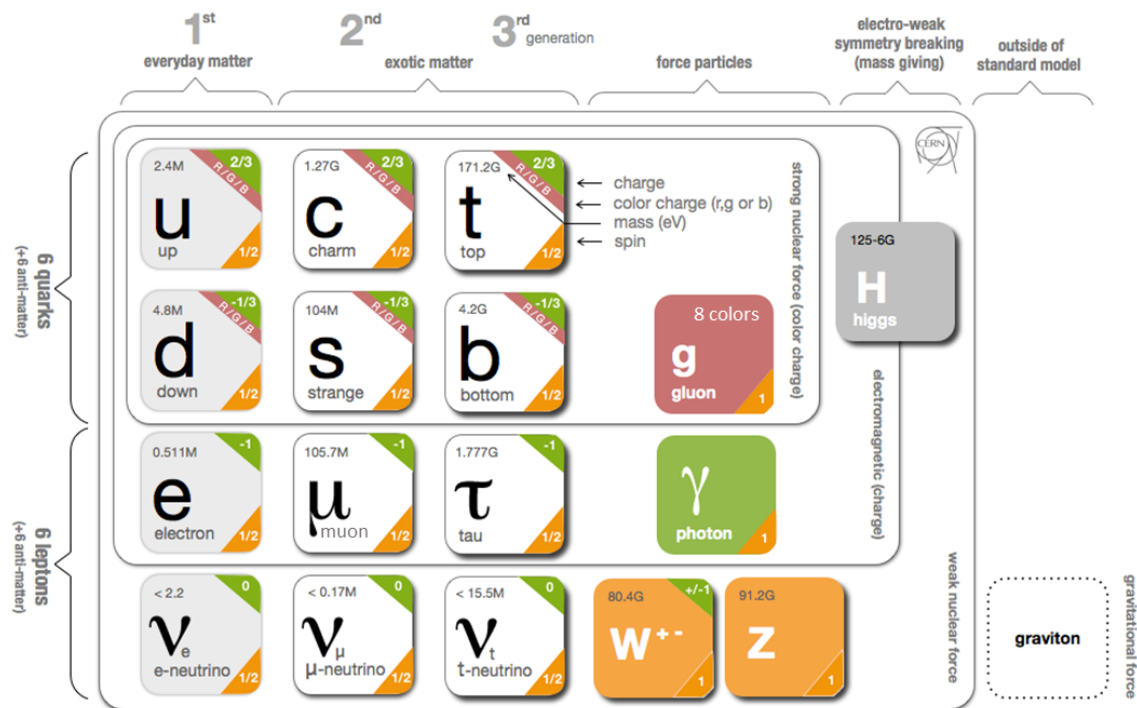
Figure 1 – Schematic view of the Standard Model of particle physics after the EW symmetry breaking [16].
