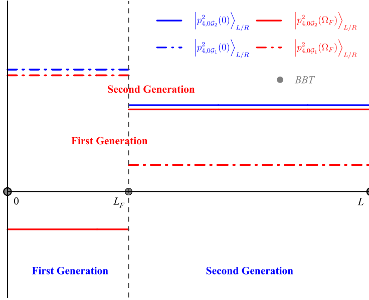
Figure 6.3 – Two pairs of profiles corresponding to \langle y | p_{4,0G_i}^2(0) \rangle_{L/R} ( i = 1, 2 ) (6.48) and \langle y | p_{4,0G_i}^2(\Omega_F) \rangle_{L/R} ( i = 1, 2 ) respectively, before and after a rotation of angle \Omega_F in Eq. (6.50), which exactly matches the rotation in the Hilbert space visualized in Figure 6.2 (same solid/dash-dot and color codes are used).
