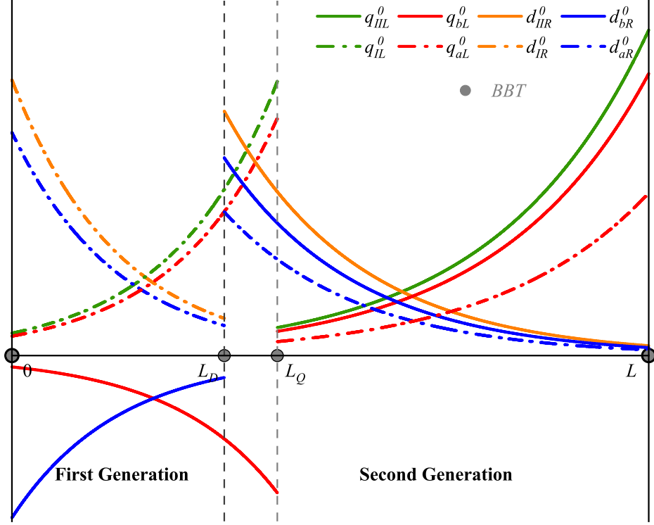
Figure 6.6 – Two ortho-normalized (6.38) generations of SM-like zero-mode wave functions, f_{\mathcal{G}_{1(2)}L/R}^0(y) [ \mathcal{G}_{1(2)} = I(II), a(b) , f = q, d ], obtained by two sets of SM-like BBT configurations \sigma_1^Q, \sigma_2^D (6.7) respectively along the entire domain, \mathcal{I}_1 = [0, L_F] \cup (L_F, L] ( F = Q, D ), corresponding to the free solutions of Eq. (6.74)-(6.75) in the simplified case, \alpha_F^{10} = \alpha_F^{20} = \delta_F = 0 , bulk masses \tilde{m}_F^i < 0 ( i = 1, 2 ).
