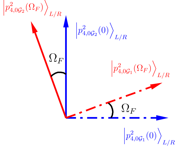
Figure 6.2 – Basis rotation (6.48) in the 0-mode Hilbert space with respect to a rotation angle \Omega_F (6.50).
