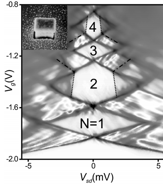
Fig. 1.11: Measured stability diagram of a quantum dot at the bath temperature of 15 mK . Dotted lines have been superimposed to highlight the onset of inelastic cotunneling. The dot-dashed lines indicate the onset of first-order tunneling via an excited state. Inset: scanning electron micrograph of the device. Adapted from [87].
