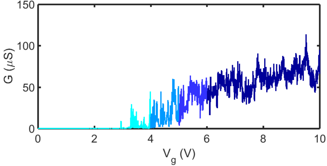
Fig. 5.2: Composite of sequential conductance measurement as a function of back gate voltage ( V_g ), distinguished by different colors from depletion of the wire ( V_g < 2.9 V) to clear Coulomb oscillations ( V_g > 4 V) and high conductance.
