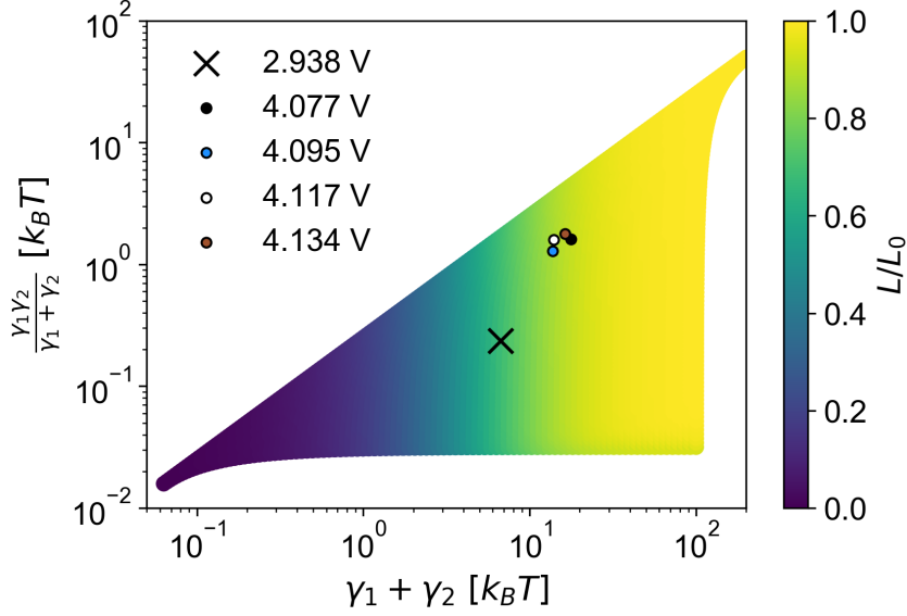
Fig. 5.14: Calculated L/L_0 on resonance as a function of the width ( \gamma_1 + \gamma_2 ) and amplitude ( \frac{\gamma_1 \gamma_2}{\gamma_1 + \gamma_2} ) of \mathcal{T}(E) . Markers show the theoretical predictions for the resonances studied in this chapter, as indicated by the legend.
