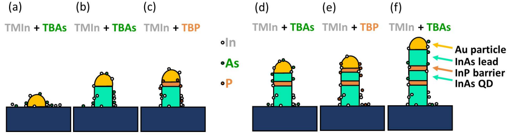
Fig. 2.3: Illustration of InAs/InP nanowire growth process. (a) Nucleation: a gold seed particle is deposited on the growth substrate. TMIn and TBAs are supplied in the growth chamber providing In and As atoms that alloy with the gold seed particle. The growth of the InAs nanowire starts when the gold particle is supersaturated with In and As atoms. Then the InAs crystal precipitates at the interface between the seed particle and the growth substrate. (b) InAs growth: Continued supply of TMIn and TBAs in the growth chamber provides In and As atoms for continued growth of InAs. (c) When the length of the first InAs segment is sufficient, the group-V precursor is switched from TBAs to TBP and InP is grown instead. (d) Once an InP barrier of the appropriate length has been grown, the precursor is switched back to InAs growth: The TBP supply is cut and TBAs is supplied in the chamber again. The InAs growth follows the description in (b) and (c).
