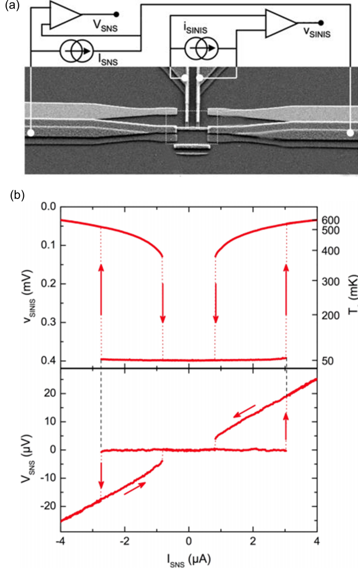
Fig. 3.6: Adapted from [138]. (a) The SEM image of the device showing an S-N-S junction of 1.5 \mu m length with a sketch of the measurement circuit. Two tunnel probes in series form SINIS structure in the middle are connected to the normal metal embedded between two superconducting banks (on the left and right sides of the image). (b) The current-voltage characteristics of the S-N-S junction device (bottom panel) shown on the same current scale with the S-I-N-I-S thermometer voltage response (top panel) was measured simultaneously at a 50 mK cryostat temperature. In the top panel, the right vertical axis gives the corresponding electron temperature .
