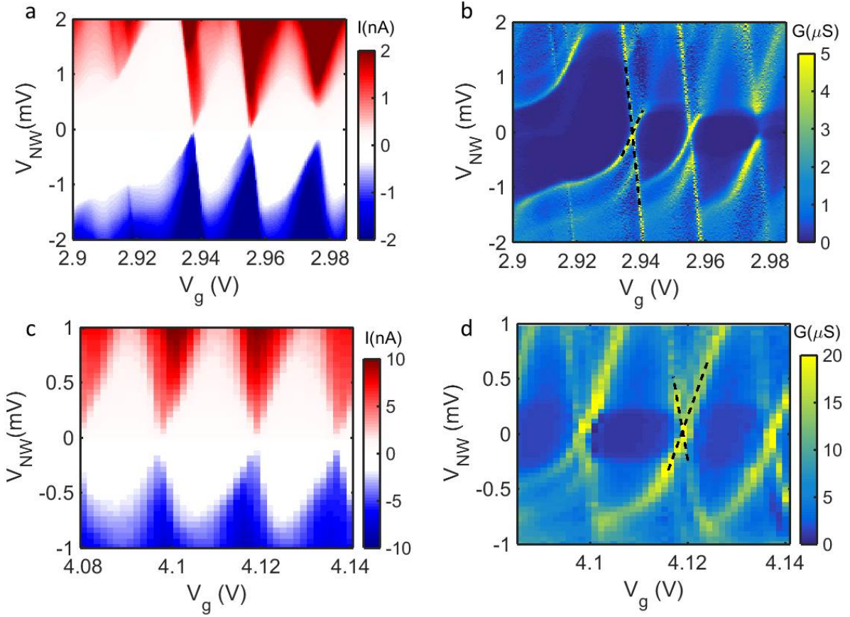
Fig. 5.3: Color map of current and conductance measurement for V_g = 2.9\text{V} and V_g = 4\text{V} showing clear Coulomb diamond structure. Additional slanted lines indicated by yellow colors in conductance map (b) and (d) outside the Coulomb diamonds display quantum dot levels excitations.
