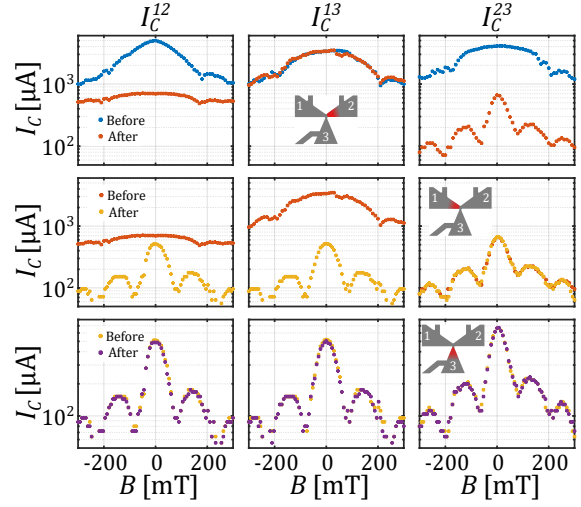
Fig. 3 Field-dependent critical currents obtained at 1.8 K through the junctions 1-2 (leftmost column), junctions 1-3 (central column) and junctions 2-3 (rightmost column) before and after EA. In the upper row, the blue dots correspond to the pristine sample and the red dots to the response after junction 2 has been modified by EA. In the middle row, junction 1 is addressed whereas in the lower row it is the junction 3 which is modified.
