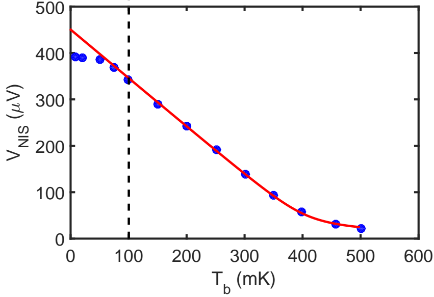
Fig. 5.6: Measured voltage across the thermometer junctions with a floating current of I_{NIS} = 5 pA as a function of the bath temperature T_b . The dashed line presents the bath temperature T_b = 100 mK used in the heat flow measurements. The red line shows the expected response of Eq. (3.9) with \Delta = 209 \mu eV and R_{T1} = R_{T2} \sim 96.2 k \Omega obtained from a similar fit as in Fig. 5.5.
