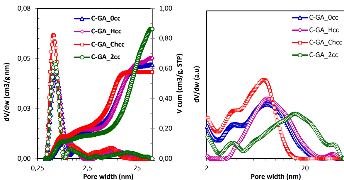
Figure 4.2.8. a) Distribution of pore sizes and cumulative pore volume evaluated using the 2D-NLDFT-HS method applied to the adsorption branch of the N_2 adsorption isotherms of the series C-GA-X-Ycc; b) magnification of the pore size distribution within the mesopore range.
