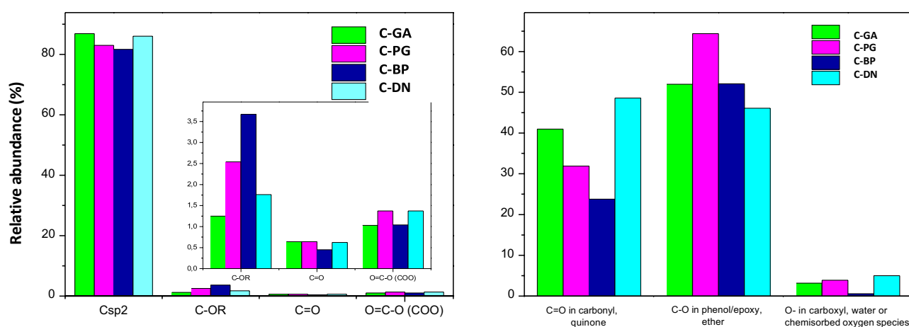
Figure 3.5. Relative abundance of carbon and oxygen species in various environments obtained by fitting the C1s and O1s core level peaks, of the carbon (left) and oxygen (right), respectively, of the XPS spectra on the prepared carbons upon carbonization at 600 °C of the photopolymerized resins.
