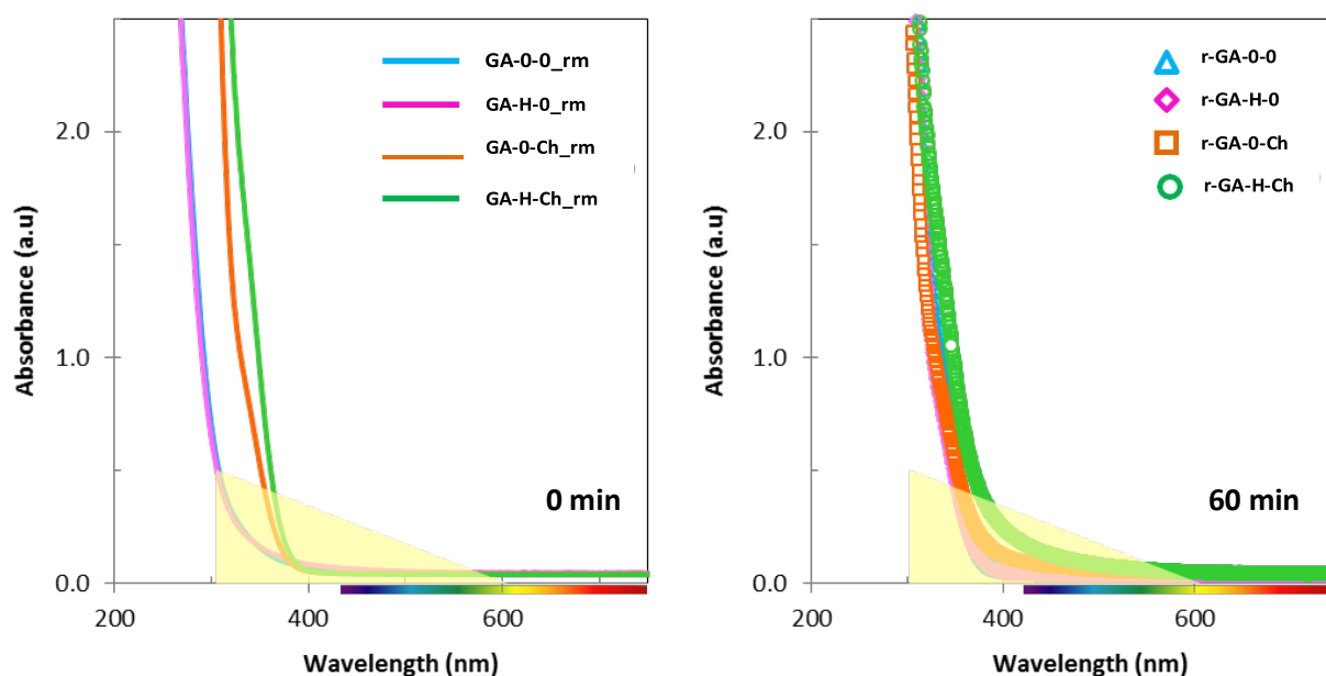
Figure 4.2.2. UV-VIS spectra of gallacetophenone reactant's mixtures before (series rm) and after 60 minutes of UV irradiation at different experimental parameters of pH and photoinitiator (series r-GA-X-Y).
