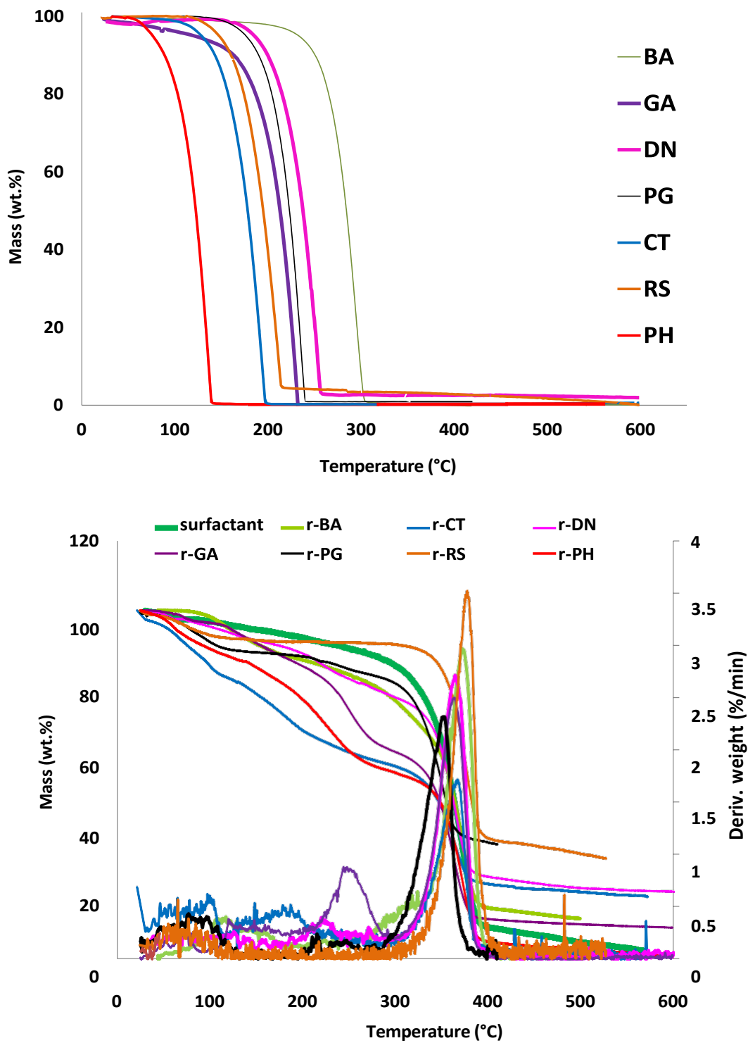
Figure 3.3. Thermogravimetric profiles under inert atmosphere of (top) the organic precursors and (down) the photopolymerized resins after 60 minutes of UV exposure (r-OP). The profile corresponding to the surfactant is included for comparison purposes.
