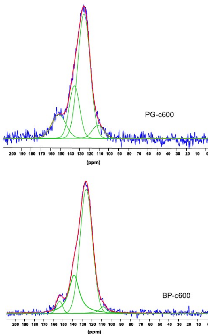
Fig. 7. ^{13}\text{C} solid-state NMR spectra of PG-c600 and BP-c600. (A colour version of this figure can be viewed online.)
