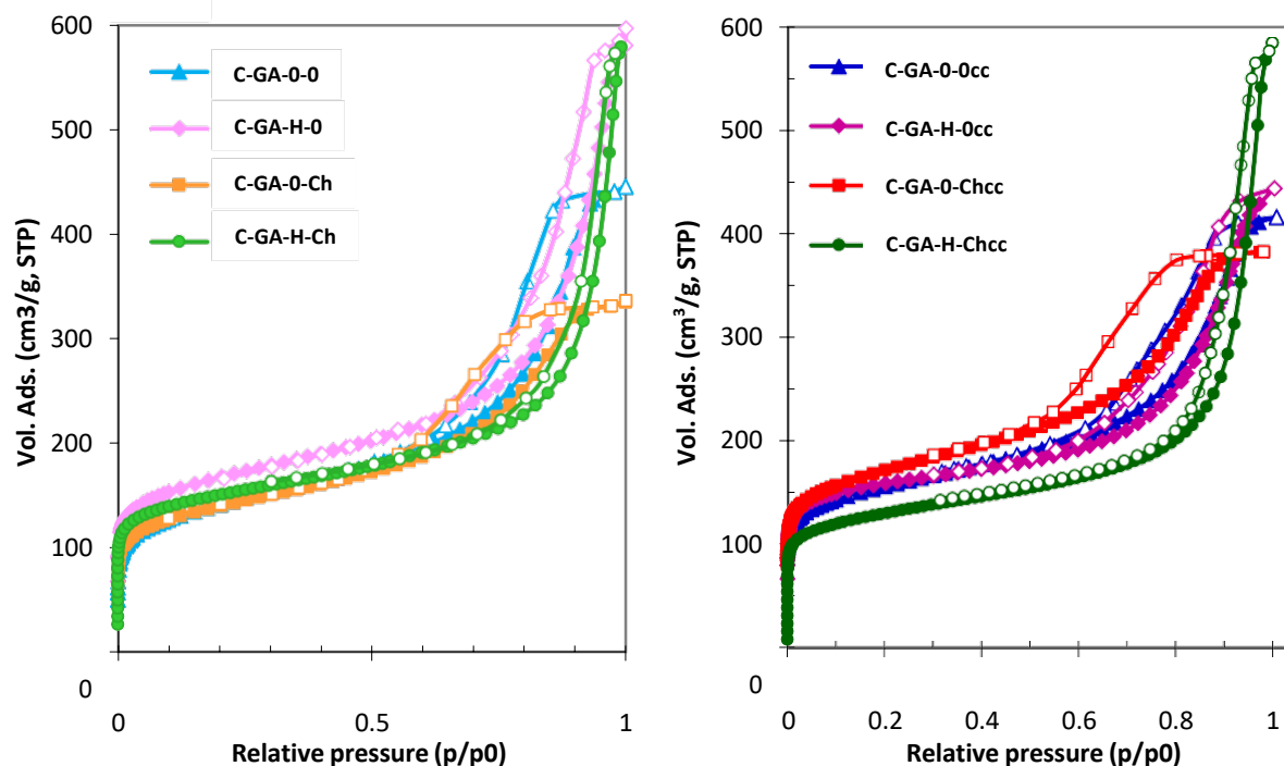
Figure 4.2.4. N 2 adsorption/desorption isotherms at -196 °C of the carbon materials obtained by the photopolycondensation of gallacetophenone at different experimental parameters of pH, photoinitiator and OP/EtOH ratio (full symbols: adsorption; empty symbols: desorption).
