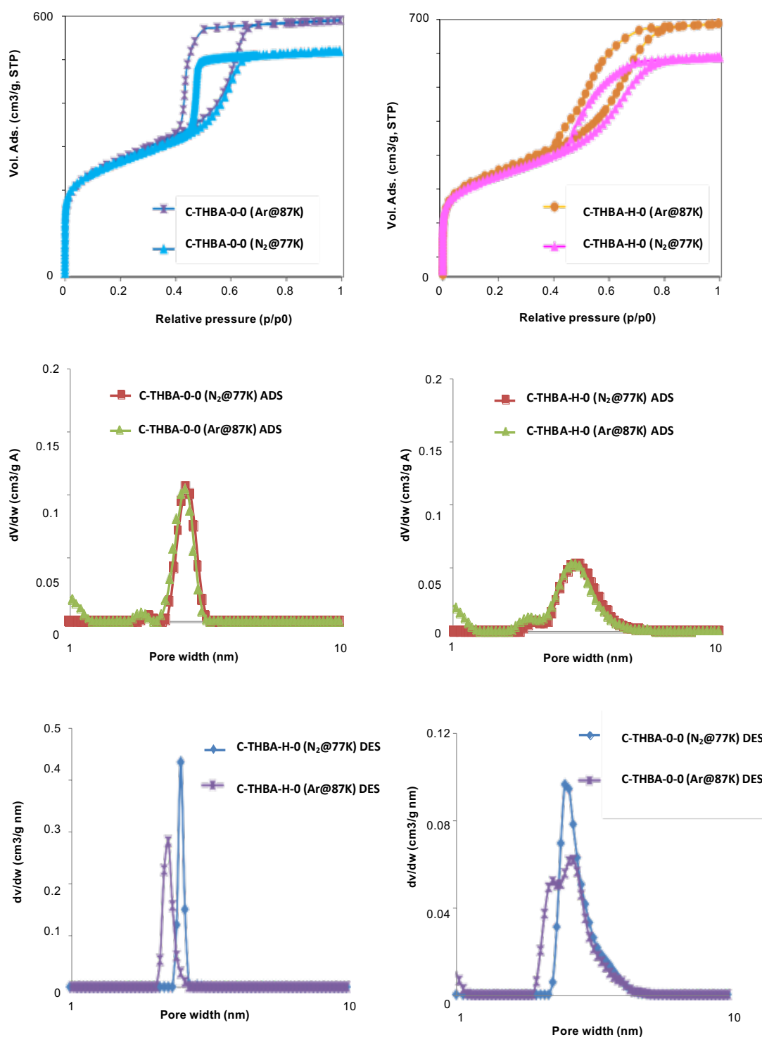
Figure 5.3.6. a) High resolution Ar adsorption isotherms at -186 °C of samples C-THBA-0-0 and C-THBA-H-0 (full symbol: adsorption branch; empty symbol: desorption branch). Data is compared to the N 2 adsorption isotherms at -196 °C; (down, left) Pore size distribution (PSD) evaluated using the QSDFT models for carbons with slit/cylinder geometry, applied to the adsorption (ADS) and desorption (DES) branches for the Ar and N 2 data.
