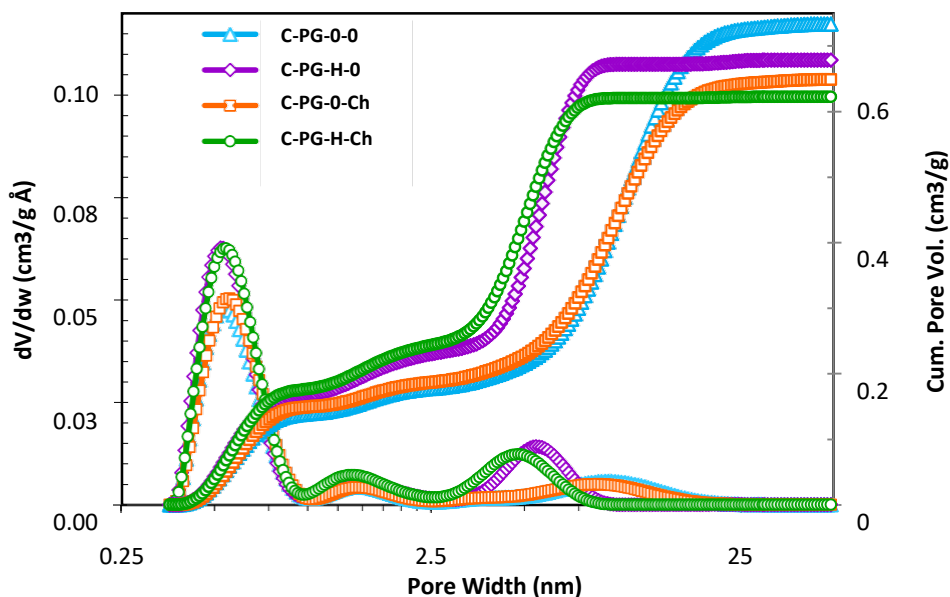
Figure 4.3.6. Pore size distribution (left -y axis) and cumulative pore volumes (right Y axis) of the carbon materials of the C-PG-X-Y series, obtained by the 2D-NLDFT-HS method applied to the adsorption branch of the N 2 adsorption isotherms at -196 °C.
