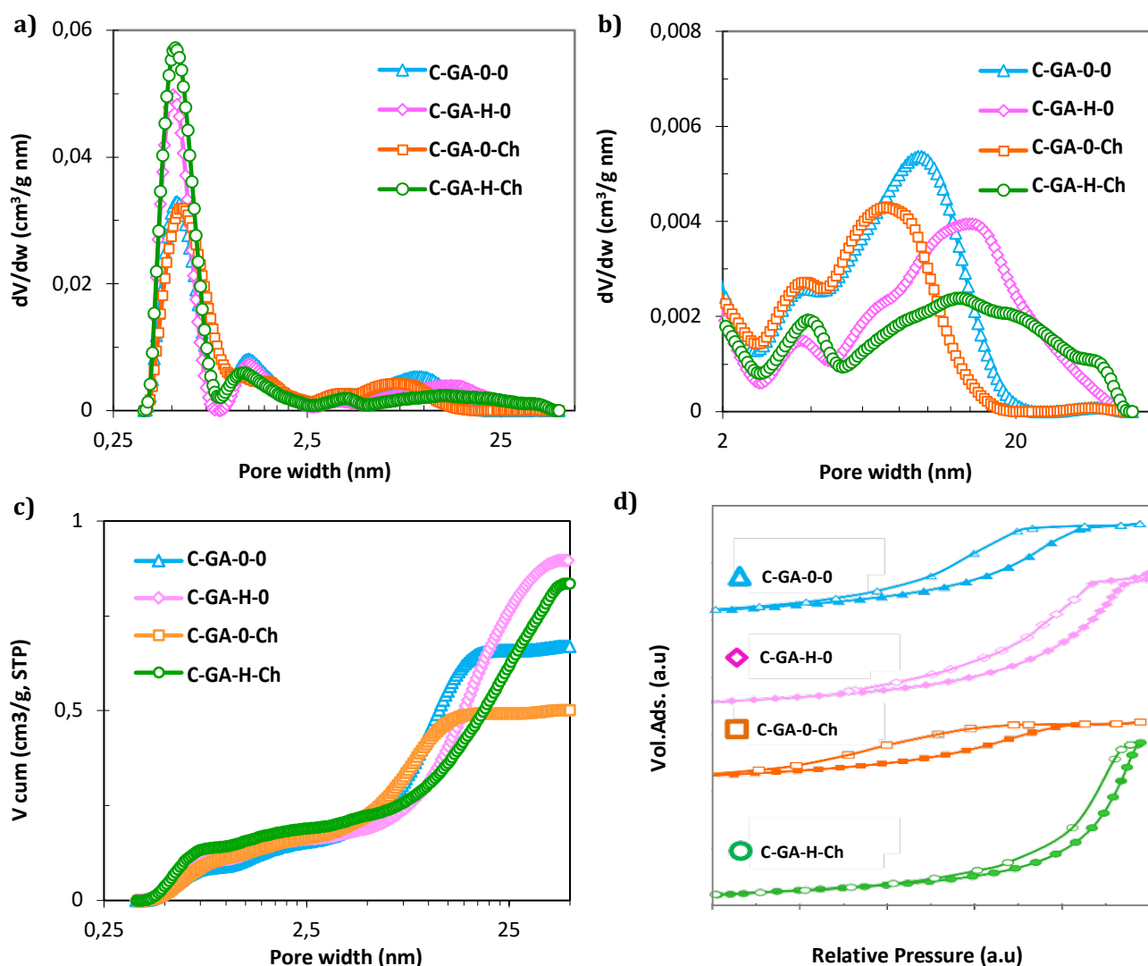
Figure 4.2.5. Derivative (a,b) and cumulative (c) distribution of pore sizes evaluated using the 2D-NLDFT-HS method applied to the adsorption branch of the nitrogen adsorption isotherms at -196 °C of the series C-GA-X-Y; (d) magnification of the hysteresis loops of the N 2 adsorption isotherms at -196 °C.
