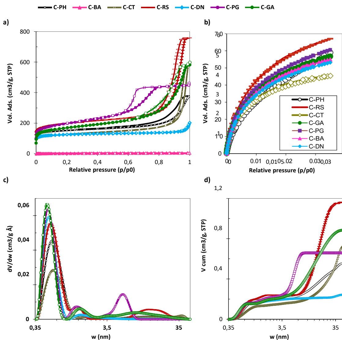
Figure 3.6. a) High resolution N 2 adsorption isotherms at -196 °C of the materials after carbonization of different photopolymerized resins from various organic precursor (full symbol: adsorption; empty symbol: desorption). b) CO 2 adsorption isotherms at 0 °C of the carbon materials. c-d) Pore size distribution (PSD) evaluated using the 2D-NLDFT-HS method from the adsorption branch of nitrogen -196 °C isotherm.
