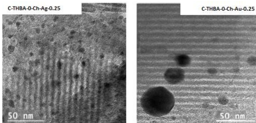
Figure 6.3.4. TEM images of the metal-loaded carbon materials prepared using THBA as precursor.
