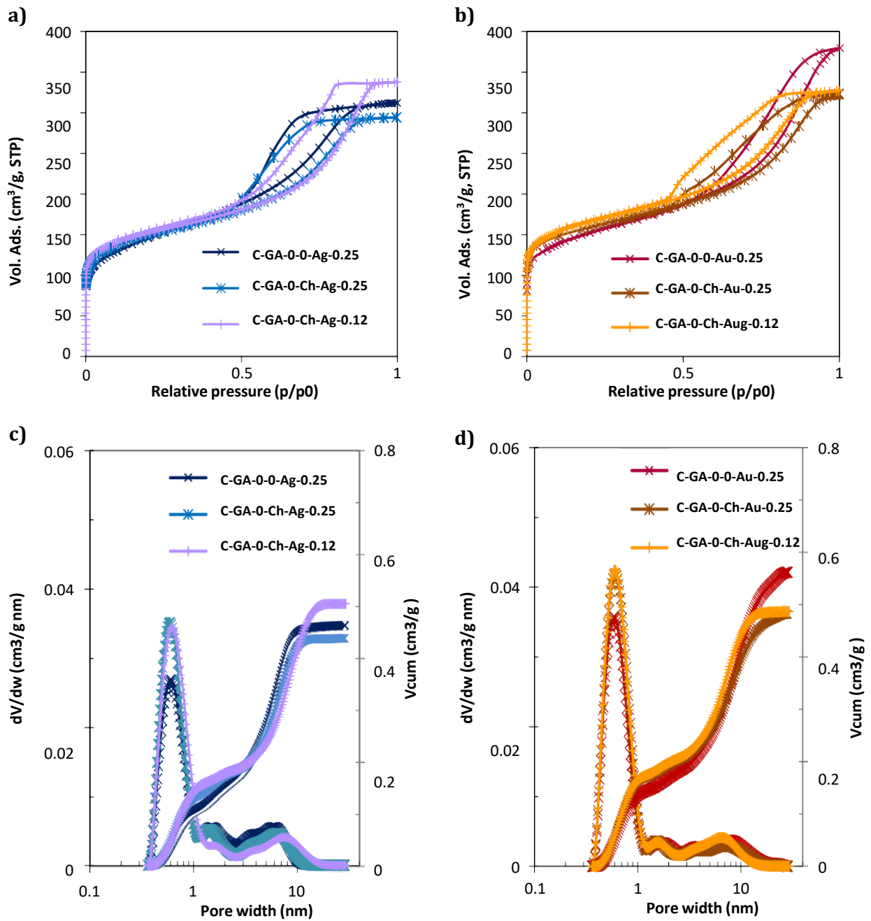
Figure 6.2.3. High resolution N 2 adsorption/desorption isotherms at -196 °C (a,b) and pore size distributions (c,d) evaluated using the 2D-NLDFT-HS method from the adsorption branch of the N 2 isotherms of the metal-containing GA series.
