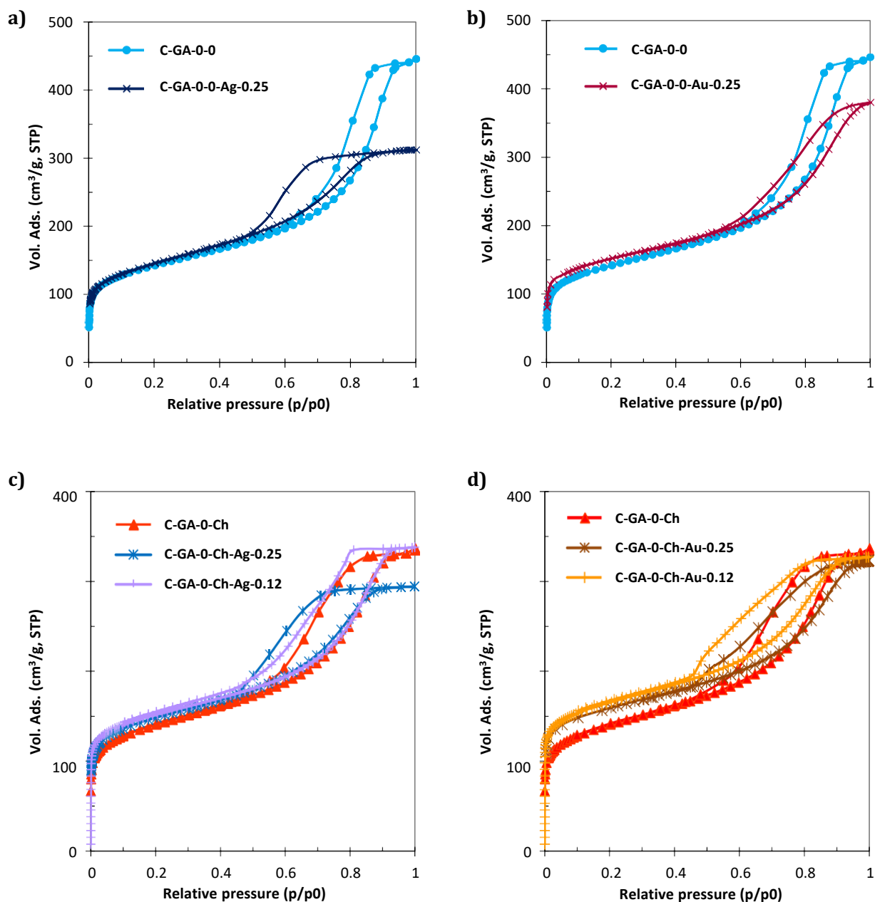
Figure 6.2.4. Comparison of the high resolution N_2 adsorption/desorption isotherms at -196\text{ }^\circ\text{C} of the samples of the C-GA series obtained in the presence and absence of metallic salts.
