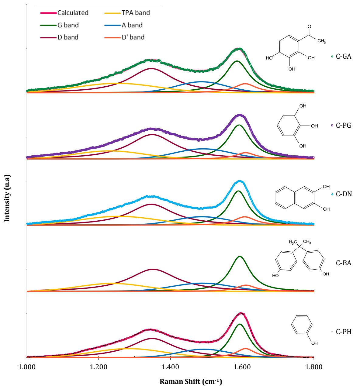
Figure 3.11. Raman profiles of the photopolymerized resins after carbonization at 600\text{ }^{\circ}\text{C} . Raw data is represented in dots; data after deconvolution and deconvoluted bands (TPA, D, A, G and D') are depicted in lines (see legends and color codes).
