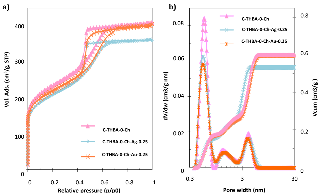
Figure 6.3.3. a) \text{N}_2 adsorption/desorption isotherms at -196\text{ }^{\circ}\text{C} of the metal-containing carbons prepared using THBA as precursor; b) pore size distributions evaluated using the 2D-NLDFT-HS method from the adsorption branch of the \text{N}_2 isotherms.
