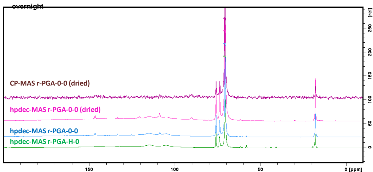
Figure 5.4.6. Comparison of the ^{13}\text{C} hpdec and CP-MAS spectra of the phenolic resins prepared using PGA as precursor.
