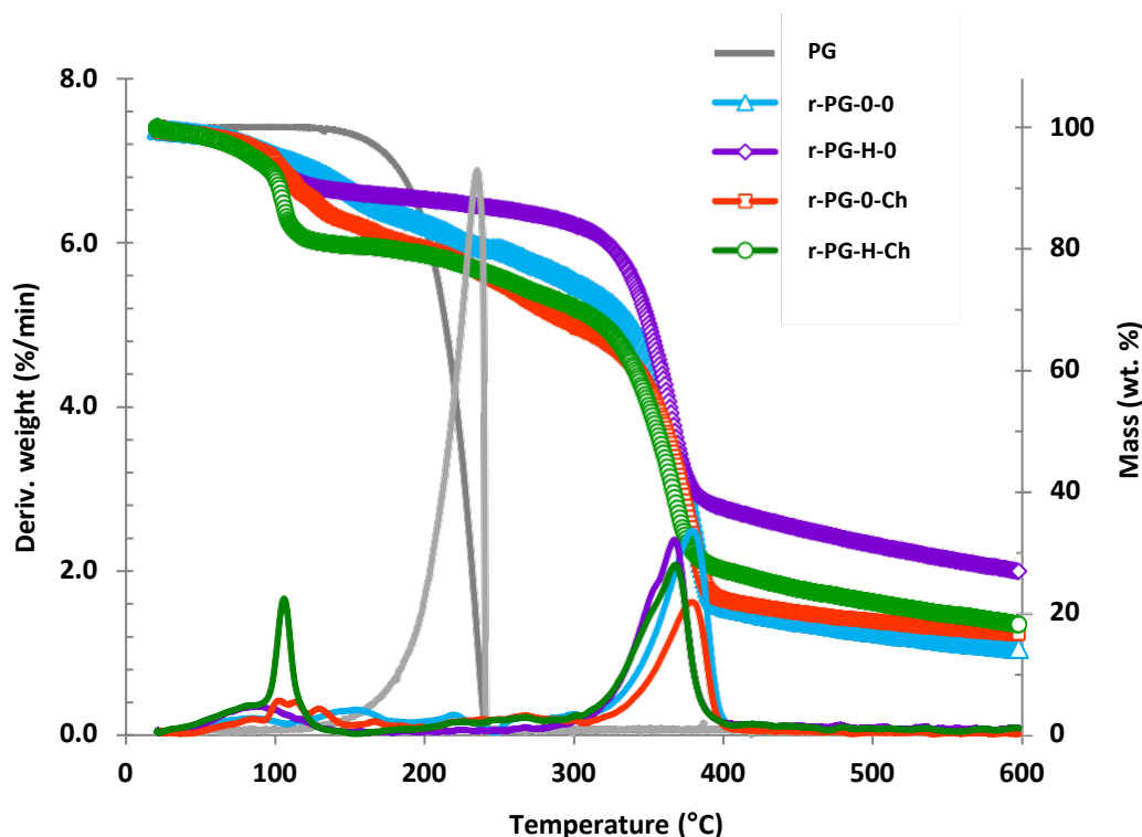
Figure 4.3.4. Thermogravimetric profiles of the series r-PG-X-Y obtained under inter atmosphere.
