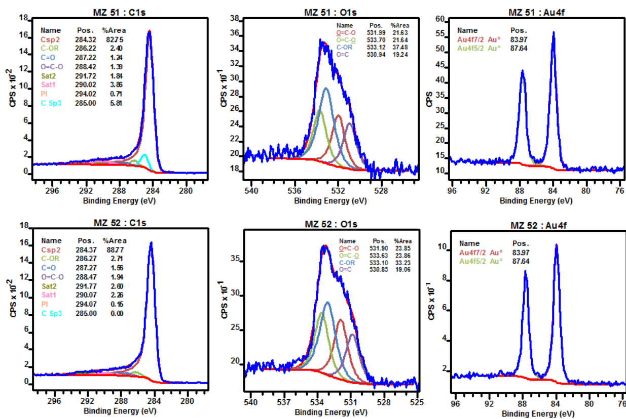
Figure 6. Experimental XPS data and fitting of the C1s O1s and Au4f core level profiles under inert atmosphere of the resins after carbonization.
