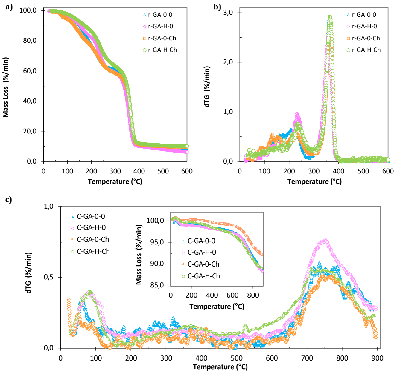
Figure. 4.2.3. a) Thermogravimetric profiles and b) derivative curves under inert atmosphere of the series r GA-X-Y after 60 min of irradiation and c) their corresponding carbons (series C-GA-X-Y) obtained upon thermal treatment at 600 °C.
