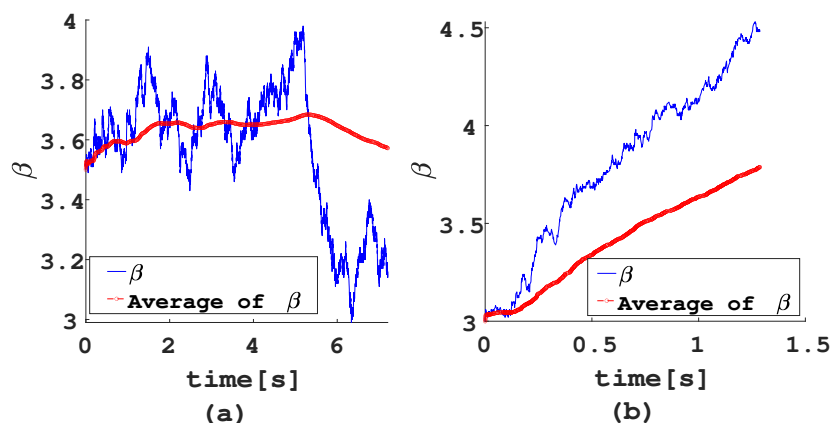
Figure 3.8: System intensity \beta as a function of time for network with truncated Gaussian beam alignment error. (a) \lambda = 0.9\hat{\lambda}_c^{BF} ; (b) \lambda = 1.1\hat{\lambda}_c^{BF} , where \sigma = 0.3 , n = 4 , \hat{\lambda}_c^{BF} = 3.7737 ( \lambda_c^{BF} = 12.9721 without misalignment).
