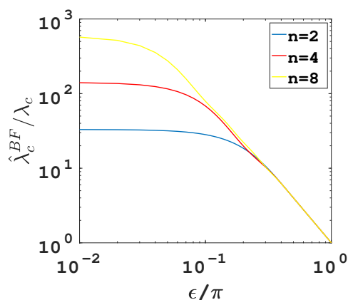
Figure 3.11: \hat{\lambda}_c^{BF}/\lambda_c as a function of \epsilon/\pi for network with Uniform beam alignment error. Figure 3.12: \hat{\lambda}_c^{BF}/\lambda_c as a function of \sigma for network with Gaussian beam alignment error.
