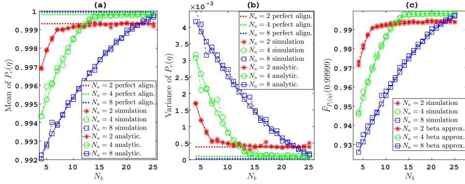
Figure 5.4: Mean (a) and variance (b) of the conditional rate coverage probability; Proportion of links that have a conditional rate coverage probability greater than a reliability threshold of 99.999% (c), as a function of the number of beams.
