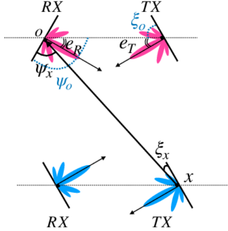
Figure 5.2: A D2D transmitter-receiver (‘TX’ and ‘RX’ in rose) at the origin o characterized by an AoD \psi_o and an AoA \xi_o . The alignment errors are denoted as e_T and e_R . An interfering D2D transmitter-receiver pair (in blue) is located in x and is characterized by an AoA \psi_x and an AoD \xi_x with respect to the rose D2D pair.
