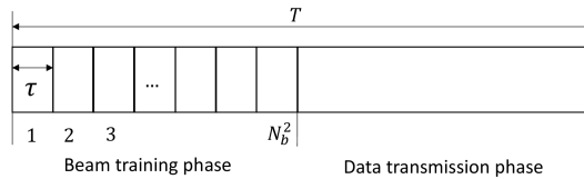
Figure 5.1: Time slot of duration T made of: (i) A beam training phase, which consists of N_b^2 mini-slots of duration \tau ; (ii) A data transmission phase.
