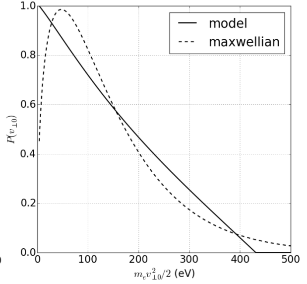
Figure 135. P(v_{\perp 0}) plotted as a function of kinetic energy for P_{in} = 20 W, \psi_g = 96 \mu\text{g/s} , E_{\mu\lambda} = 4200 V/m, \bar{\sigma} = 1.0 . The initial value is normalized to 1.
