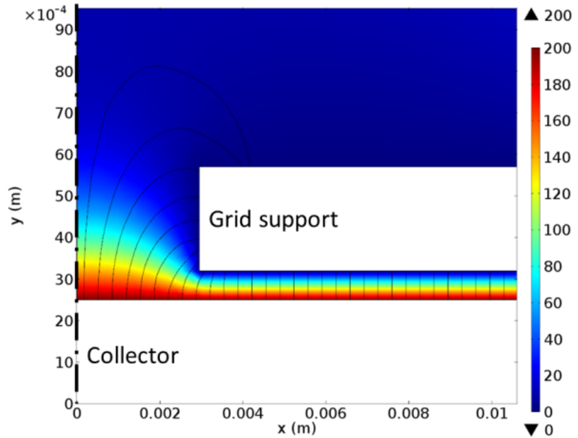
Figure 63. Electrostatic potential in V and electric field lines for the gridded Faraday probe without grid. The opening in the grid support is considered as the collector diameter.
