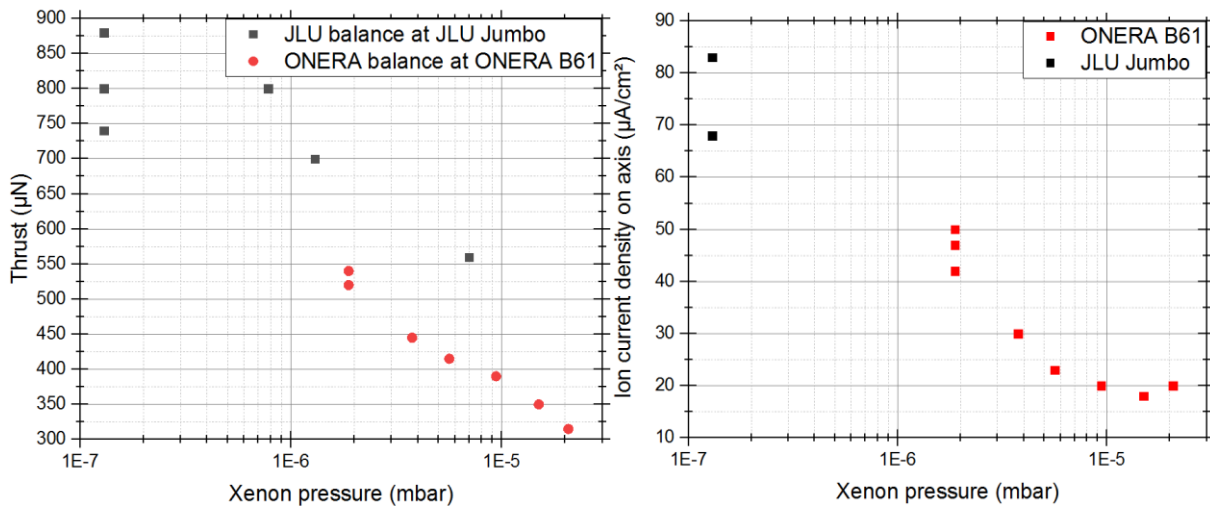
Figure 81. Thrust and ion current density. Estimations of error bars were not available for the JLU balance; ONERA error bars are of the order of the size of the dots ([24], figure 93). Ion current is measured with the gridded Faraday.
