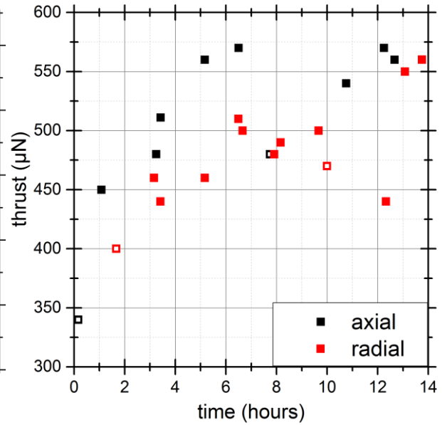
Figure 97. Thrust (thruster configuration form table 7 except for the inner conductor being covered with boron nitride spray). Hollow symbols indicate the first measurement point after startup with a cold thruster.
