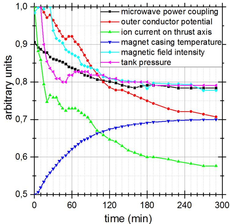
Figure 84. Transient operation of the thruster at 24 W and 1sccm. Microwave power coupling is in real scale. All other curves are arbitrarily normalized.
