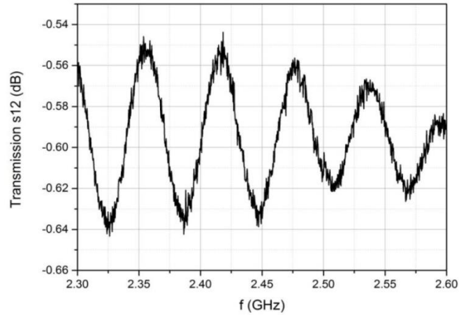
Figure 18. Typical VNA measurement of a coaxial cable (VIALIS III-2.3 [24])
