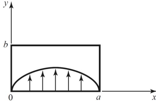
Figure 14. Electric field of the TE10 mode of the rectangular waveguide
