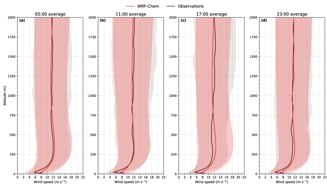
Figure B.4: Modelled and observed vertical profiles of wind speed with MOSAiC radiosondes. Mean vertical wind speed profile from radiosonde observations (black) released above the MOSAiC shiptrack and simulated by WRF-Chem (red) during the simulation period (March 14 – April 14, 2020). Model values are extracted at the closest grid cell to the location of each radiosonde flight path. Data are averaged by time interval during the simulated period (to the nearest hour) at (a) 05:00 UTC, (b) 11:00 UTC, (c) 17:00 UTC, and (d) 23:00 UTC. Shaded areas represent the standard deviation of the observed and model averages.
