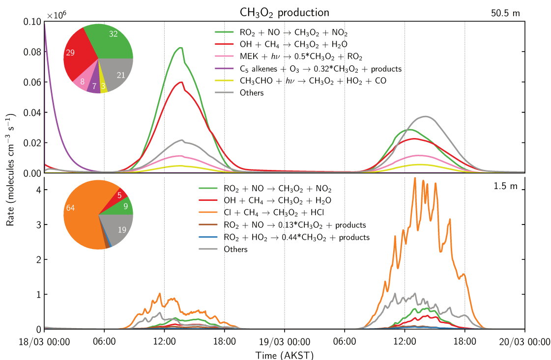
Figure 4.11: Modelled production reactions of \text{CH}_3\text{O}_2 at 1.5 m and 50.5 m above the snow surface. The five largest contributing reactions are shown for each with the percentage contributions shown as a pie chart.
