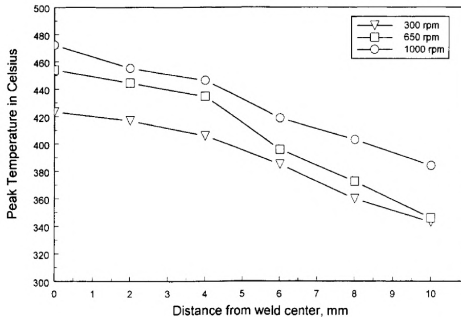
Figure I.21: Temperature profile of multiple FSW joints performed at different rotational speed in AA6061-T6 by Tang et al. [50]. An increase in rotational speed generates an increase in welding temperature.
