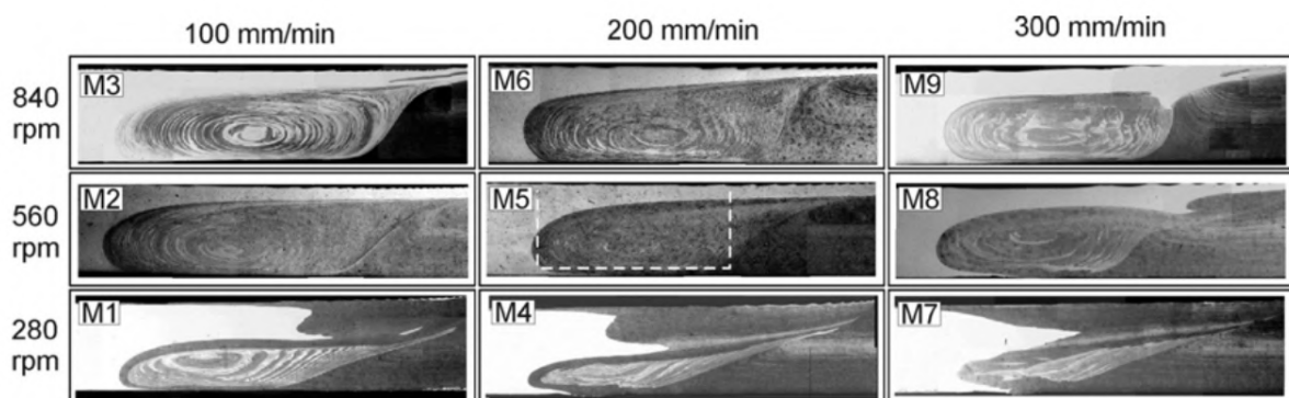
Figure I.28: Macrographs showing the influence of increasing the rotational speed on the mixing of the stir zone in a dissimilar AA5083/AA6082 weld [51].
