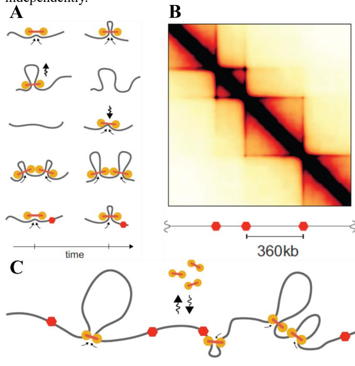
Figure 17. Loop extrusion model
