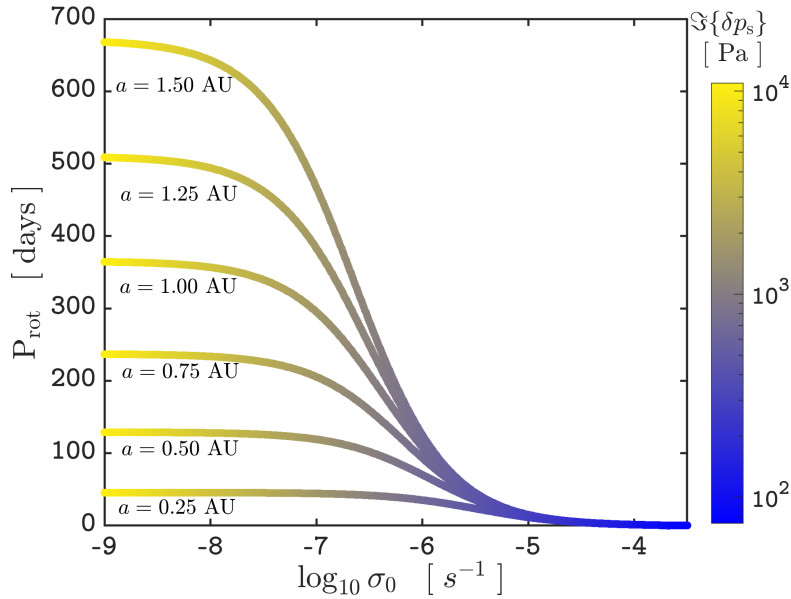
FIGURE 3.10: The position of the thermal peak near synchronization plotted in terms of the rotational period of the planet, as a function of the dissipation frequency \sigma_0 , for different values of the planetary semi-major axis (Eq. 3.120). Color coding corresponds to the amplitude of the peak.
