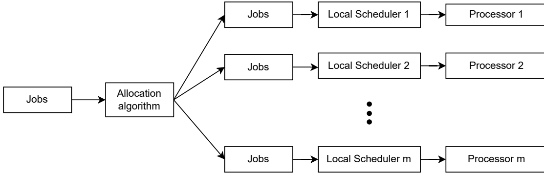
Figure 1.4: Restricted scheduling policy
