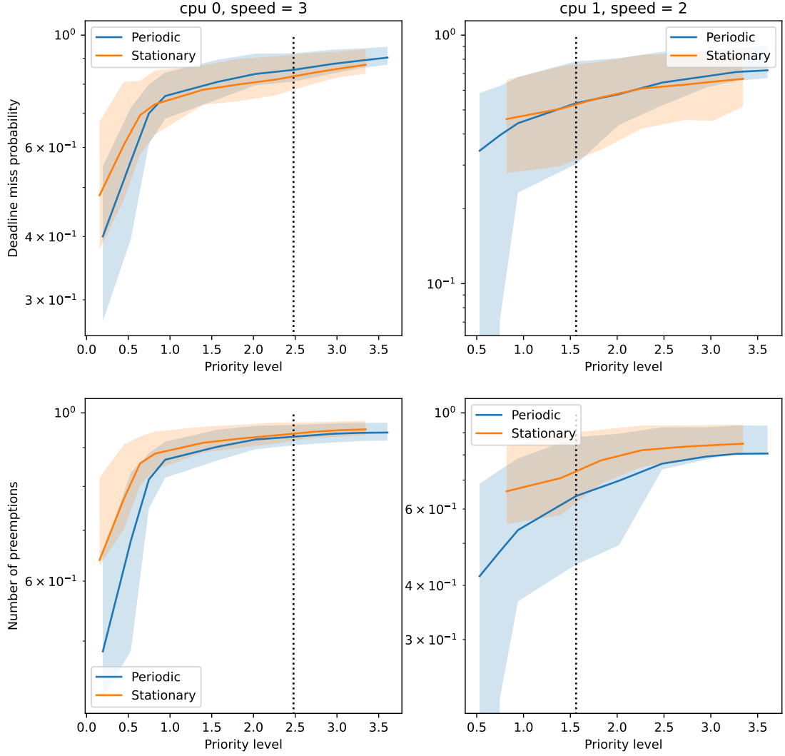
Figure 6.4: Comparison of RM-DMP-First-Fit on a stationary task set and its periodic equivalent. The first row represents deadline misses, the second row preemptions. Each column represents a processor. The dotted line represents deadline misses when the maximal local utilization exceeds 1. In solid line the average value and the colored area represent the values between the 25%-percentile and the 75%-percentile.
