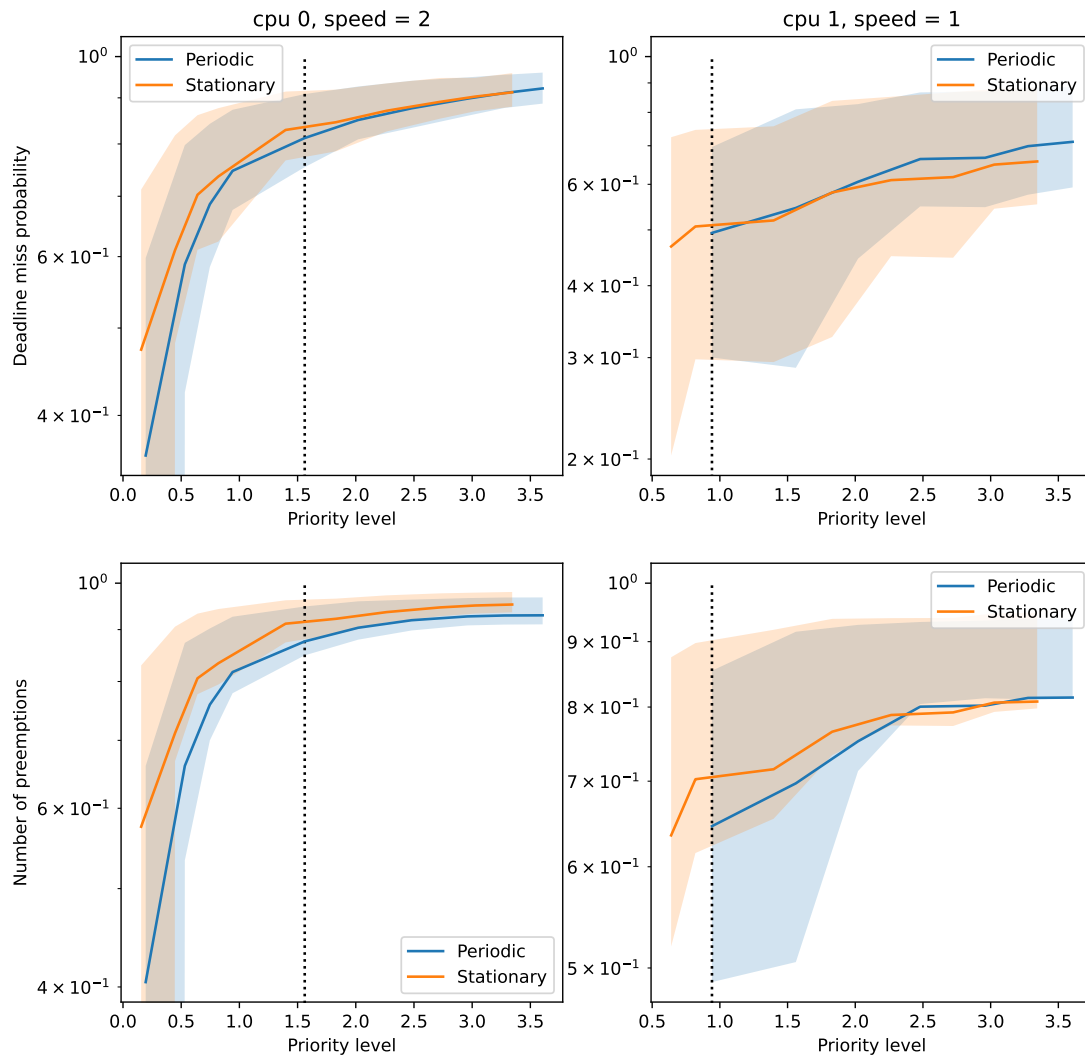
Figure 6.5: Comparison of RM-DMP-First-Fit with Hoeffding DMP on a stationary task set and its periodic equivalent. The first row represents the number of deadline misses, the second row the number of preemptions. Each column represents a processor. The dotted line represents deadline misses when the maximal local utilization exceeds 1. In solid line the average value and the colored area represent the values between the 25%-percentile and the 75%-percentile.
