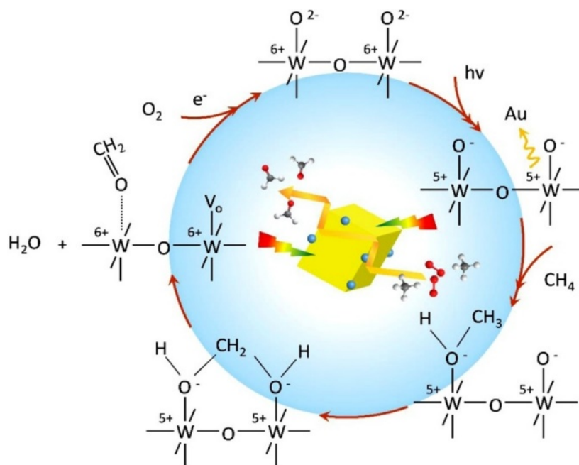
Figure 9. Proposed reaction mechanism for HCHO generation over c-WO 3
