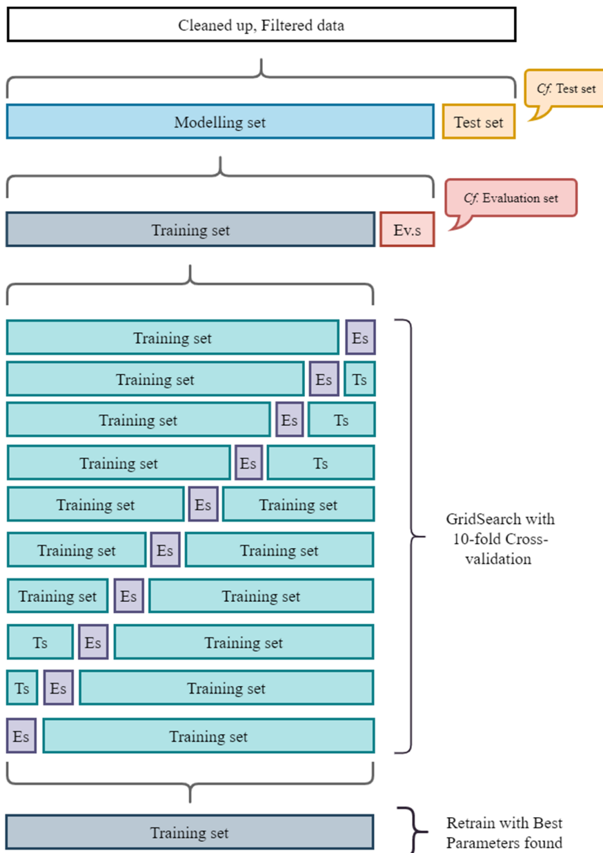
Sequence of Modelling/Testing & Training/Evaluation Data Splitting
