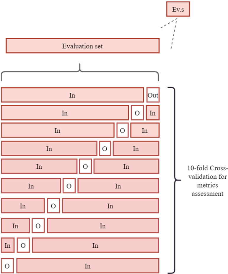
Figure 7-35 Cross Validation Task for Metrics Assessment (Evaluation)
