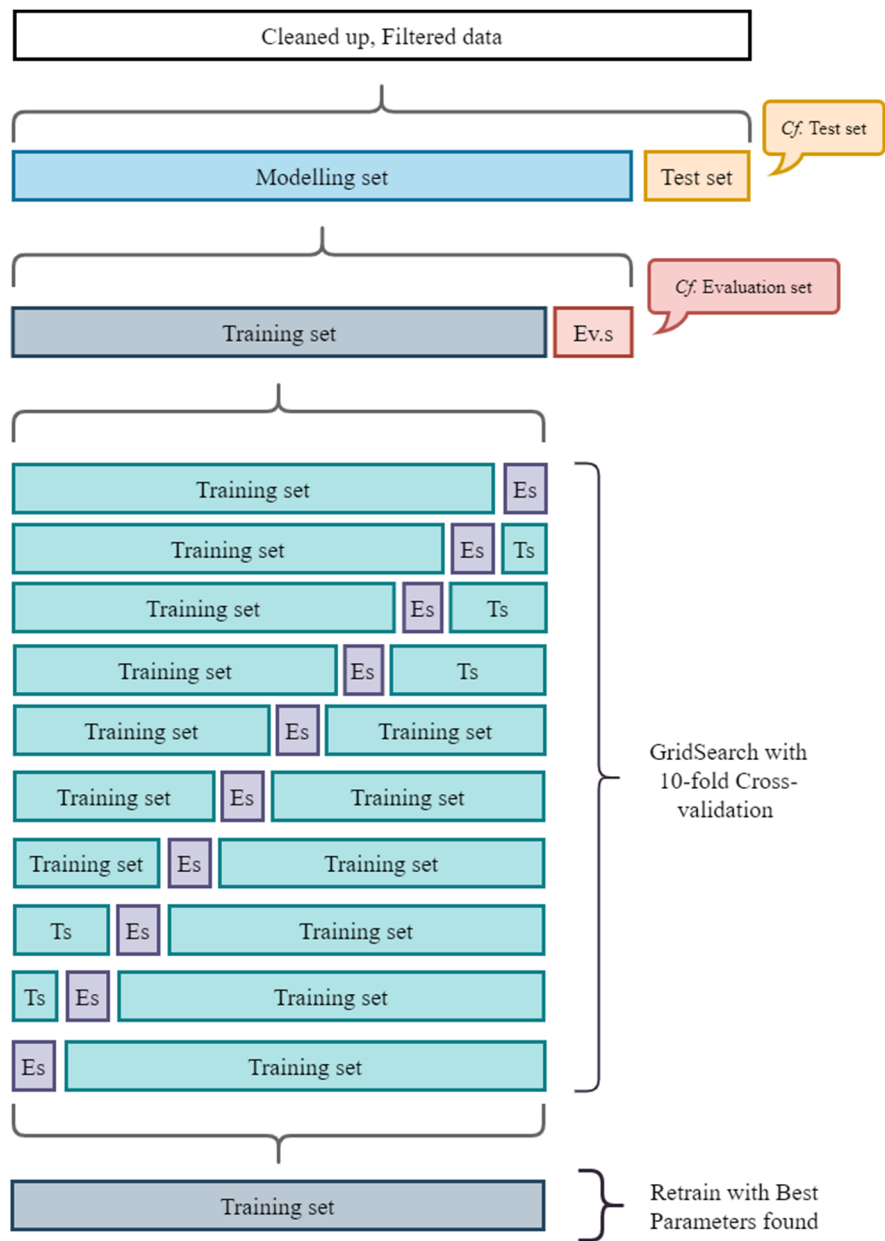
Sequence of Modelling/Testing & Training/Evaluation Data Splitting
