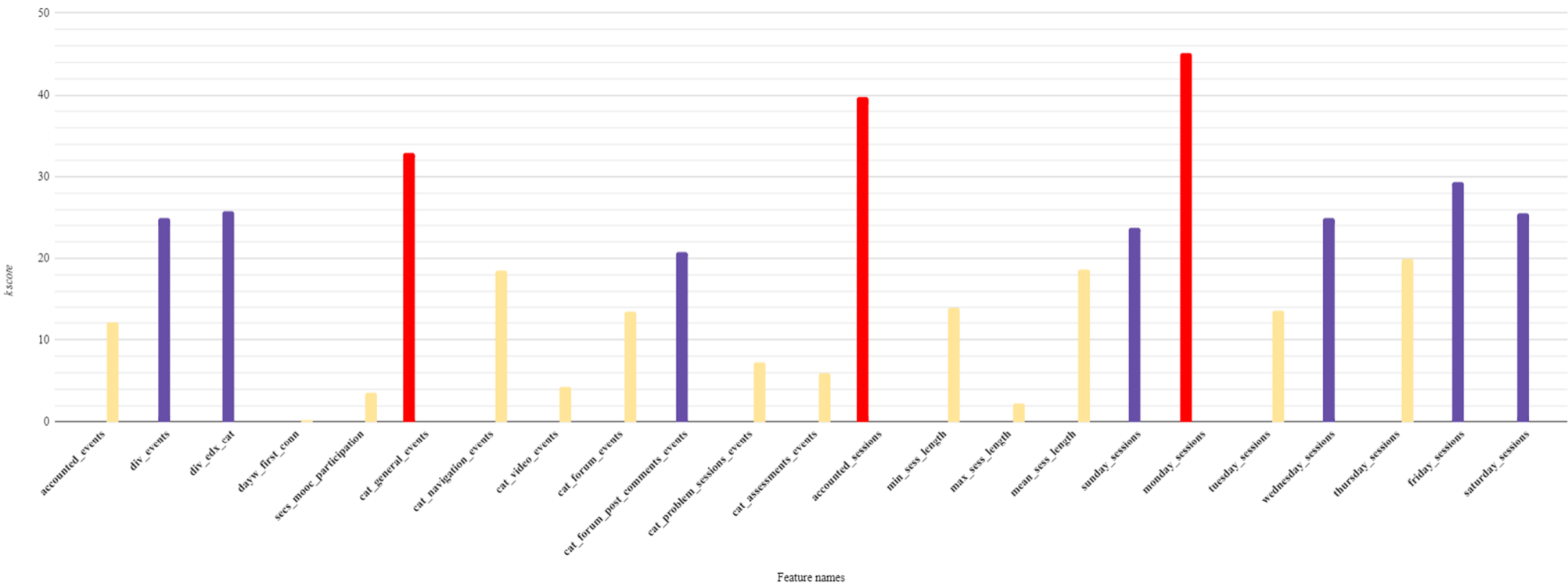
FeatureSelection k-scores
