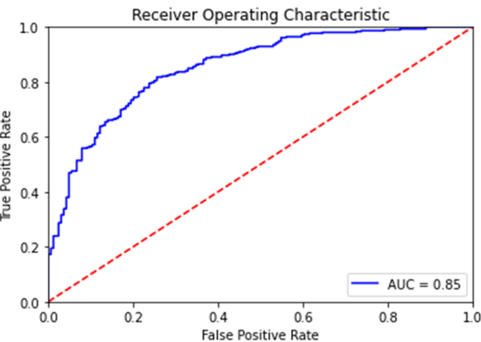
ROC Curve of the Flow-Detecting Machine Learning Model
