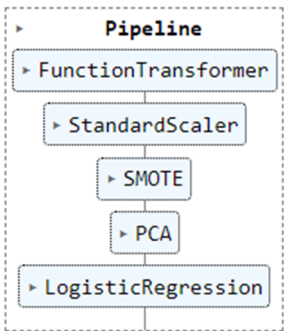
Figure 7-32 Base pipeline for Training
