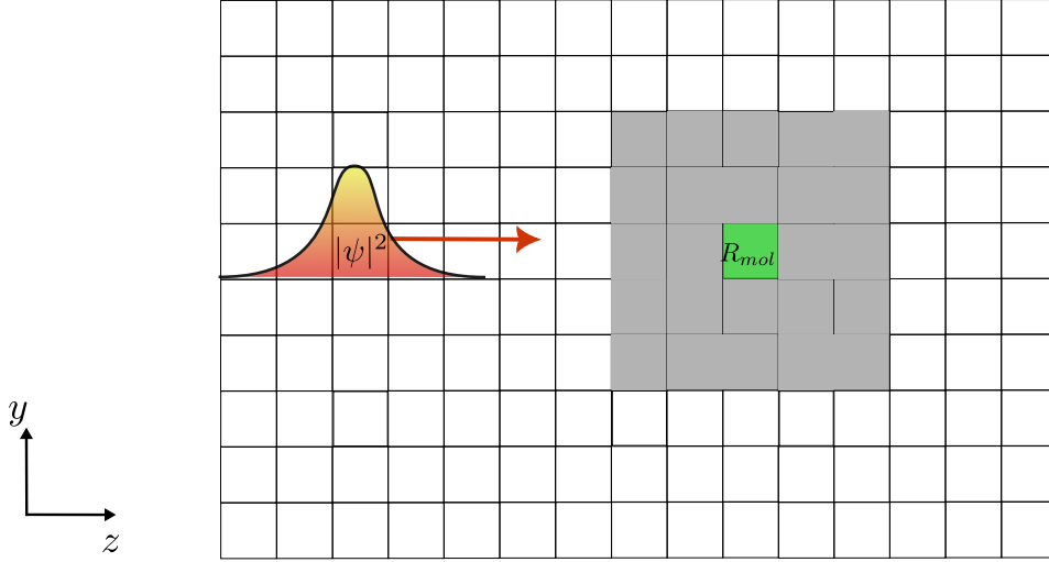
Figure 2.1: Schematic representation of a simulated system with a propagating carrier scattered on a perturbed central region.
