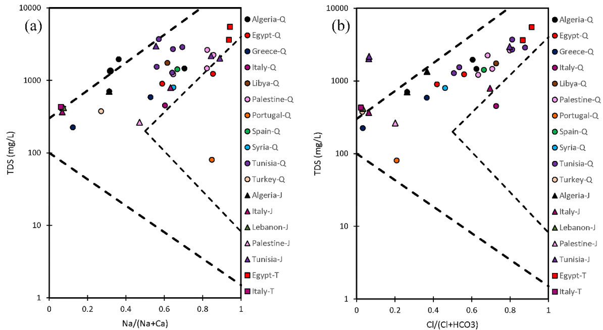
Figure 1.4 Gibbs diagrams representing; (a) TDS Vs \text{Na}^+ / (\text{Na}^+ + \text{Ca}^{2+}) and (b) TDS Vs \text{Cl}^- / (\text{Cl}^- + \text{HCO}_3^-)
