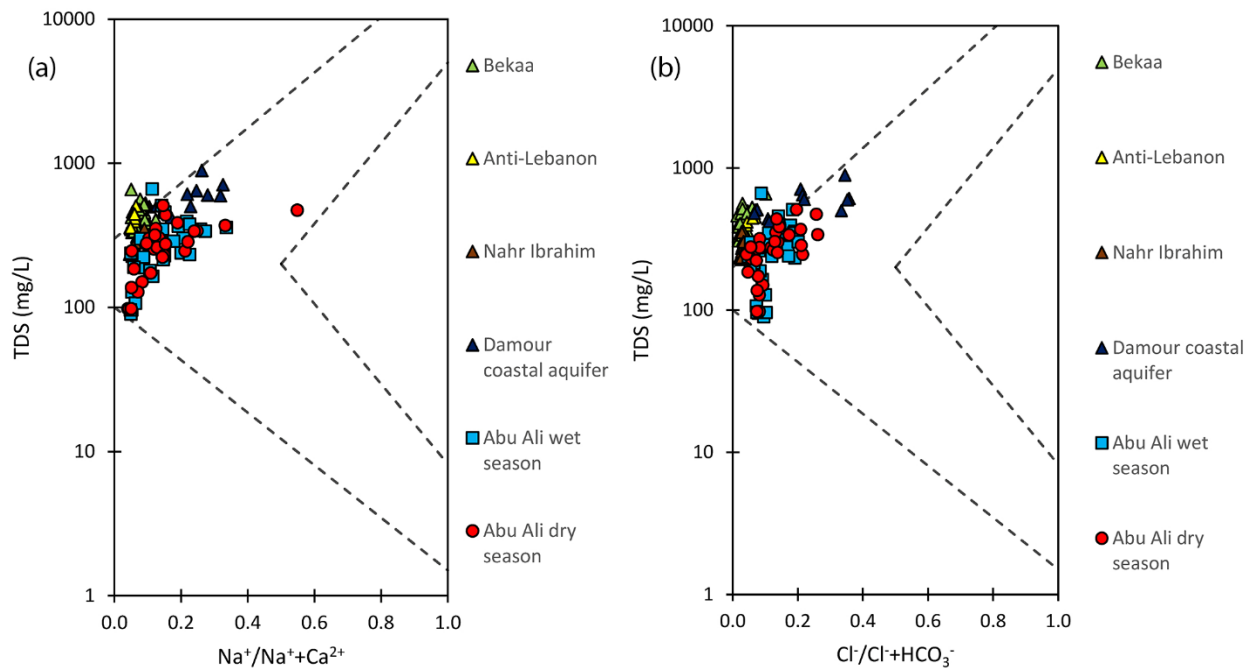
Figure 2.15 Gibbs plots of the Lebanese studies representing the variation of TDS in comparison with the ratios \text{Na}^+/\text{Na}^+ + \text{Ca}^{2+} (a) and \text{Cl}^-/\text{Cl}^- + \text{HCO}_3^- (b).
