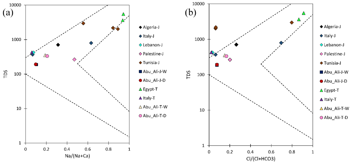
Figure 2.17 Gibbs plots of the Mediterranean studies representing the variation of TDS in comparison with the ratios Na^+/Na^+ + Ca^{2+} (a) and Cl^-/Cl^-+HCO_3^- (b). The data was divided based on the countries and the 2 main aquifers' types: Jurassic & Cretaceous and Tertiary. (Abbreviations in the legend: J "Jurassic & Cretaceous", T "Tertiary", W "Wet season", D "Dry season").
